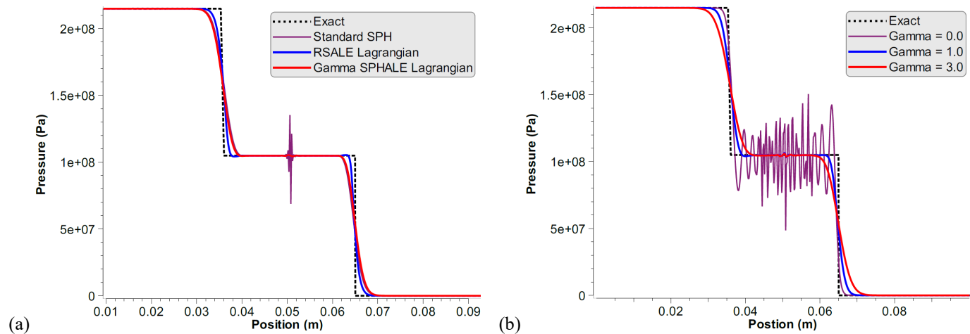
Fig. 1. Shock Tube Pressure fields comparisons at t = 10^{-5}\text{s} (a) for several schemes ( \gamma=1.0 for Gamma SPHALE), (b) for \gamma -SPH-ALE with several values of \gamma .
