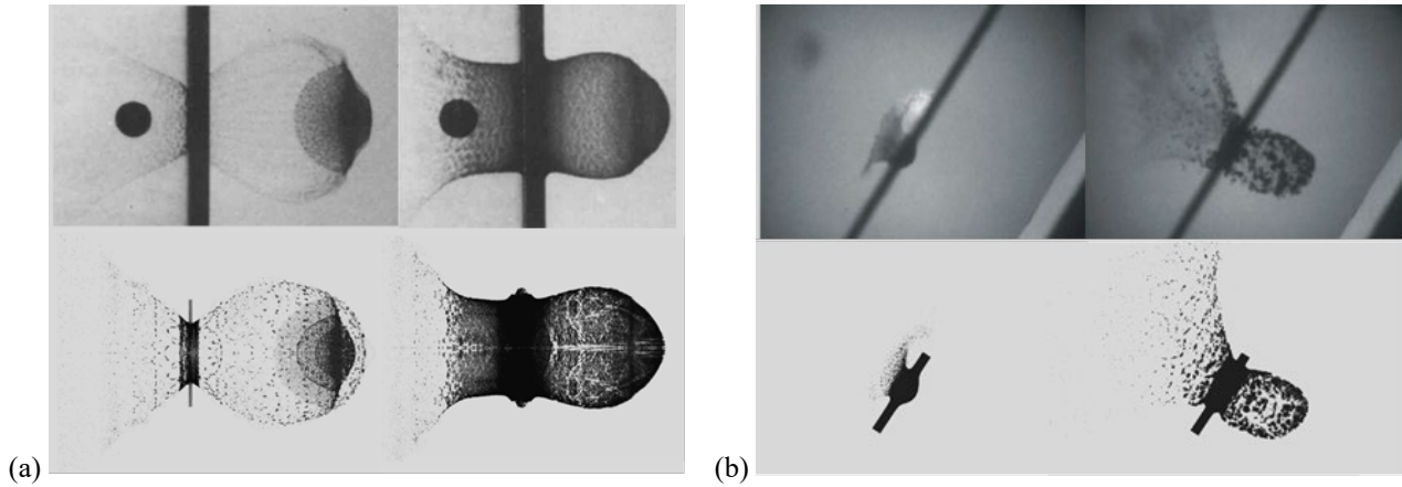
Fig. 2. Hypervelocity Impact Comparison between experiments (top) and \gamma -SPH-ALE (bottom) (a) normal impact Thickness = 0.8mm (left), Thickness = 4.039 mm (right), (b) oblique impact.
