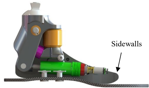
Figure 8. Single-axis design with horizontal cylinder and optimized bumper location.
