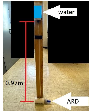
FIGURE 3: VALIDATION TEST SETUP FOR ARD V3.
