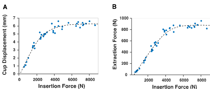
FIGURE 2: (A) INSERTION FORCE VERSUS CUP DISPLACEMENT FOR DROP TESTING (SMOOTHING SPLINE FIT, R^2 = 0.957 ). (B) INSERTION FORCE VERSUS AXIAL EXTRACTION FORCE FOR DROP TESTING (SMOOTHING SPLINE FIT, R^2 = 0.981 ).
