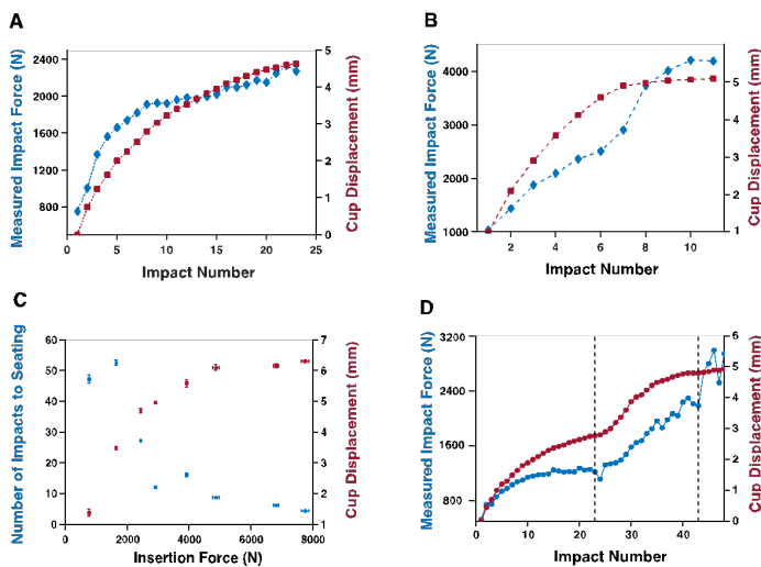
FIGURE 1: (A) THE RELATIONSHIP OF IMPACT FORCE EXPERIENCED IN THE CAVITY VERSUS CUP INSERTION FOR A 50 MM WEIGHTED DROP TEST. (B) THE RELATIONSHIP OF IMPACT FORCE EXPERIENCED IN THE CAVITY VERSUS CUP INSERTION FOR A 90 MM WEIGHTED DROP TEST. (C) NUMBER OF IMPACTS TO ACHIEVE PLATEAUED CUP INSERTION (NOITS) VERSUS INSERTION FORCE PER IMPACT. (D) PROOF OF PRINCIPLE WITH THREE GRADUATED APPLICATIONS OF DROP HEIGHT FORCES (INDICATED BY BLACK DASHED LINES).
