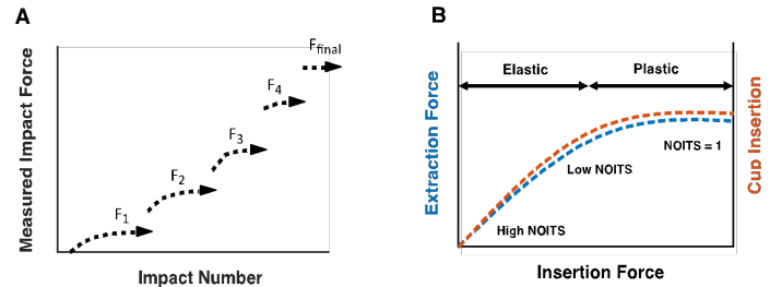
FIGURE 3: CONCEPTUAL REPRESENTATION OF: (A) THE RELATIONSHIP BETWEEN IMPACT NUMBER AND PLATEAUING VALUES OF MEASURED IMPACT FORCE FOR A GRADUATED SET OF APPLIED FORCES AND (B) THE RELATION BETWEEN NUMBER OF IMPACTS TO SEATING (NOITS) AND CUP INSERTION, EXTRACTION FORCE.
