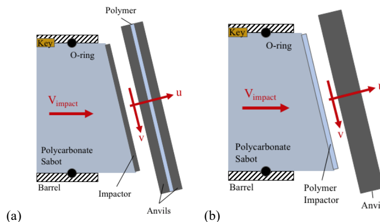
Fig. 1. Oblique impact experiment configurations (a) A CPPSPI experiment which consists of an angled projectile planarly impacting a target package set at an angle of obliquity. The target package consists of a front anvil, polymer sample, and rear anvil respectively. Note a key is shown which maintains projectile orientation down the slotted-barrel. (b) A dynamic friction impact experiment, wherein the same angled planar impact is facilitated, however the polymer of interest serves as the impactor.
