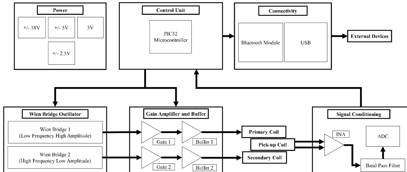
Figure 3. MPS device circuit board design block diagram.
