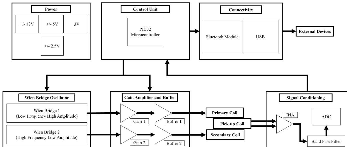
Figure 3. MPS device circuit board design block diagram.
