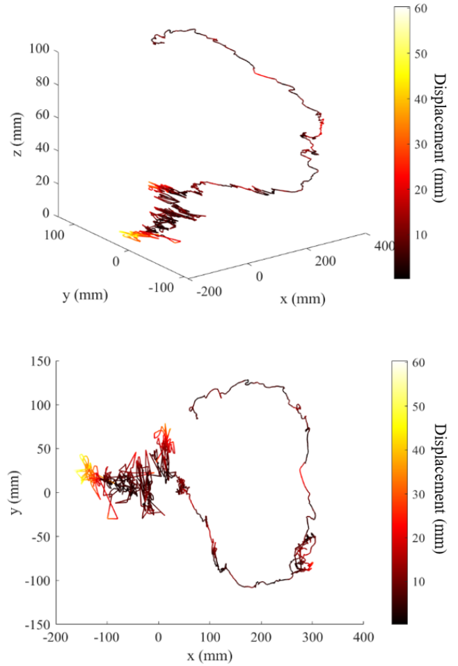
FIGURE 3: PATH DEFLECTION COLOR MAP BETWEEN INSERTION AND RETRACTION IN XYZ PLOT (TOP) AND XY PLOT (BOTTOM).
