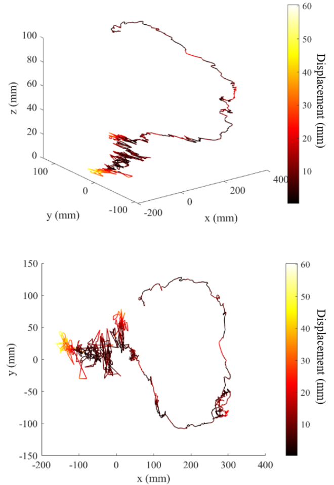
FIGURE 3: PATH DEFLECTION COLOR MAP BETWEEN INSERTION AND RETRACTION IN XYZ PLOT (TOP) AND XY PLOT (BOTTOM).
