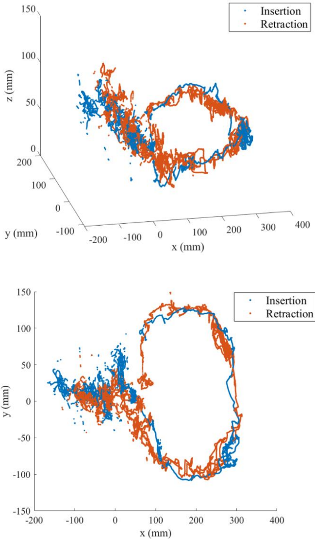
FIGURE 2: THREE-DIMENSIONAL PLOT OF PATH TRACKED BY MAGNETIC TRACKER IN COLON MANIKIN (TOP). TWO-DIMENSIONAL PLOT OF PATH TRACKED BY MAGNETIC TRACKER IN COLON MANIKIN (BOTTOM).
