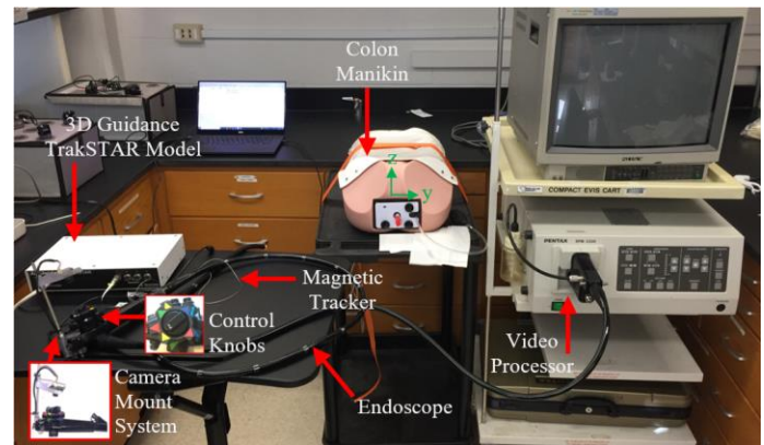
FIGURE 1: SETUP OF ECAS FOR THE ENDOSCOPIC DATA COLLECTION IN HERSHEY MEDICAL CENTER
