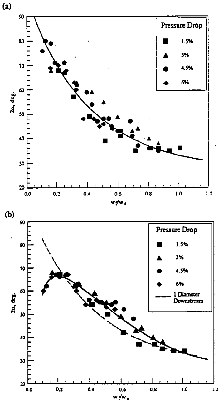
Figure 7. Spray angle measured downstream of the nozzle as a function of nozzle fuel/air ratio and nozzle air pressure drop at 10 atm. air pressure: (a) one diameter, and (b) two diameters downstream of the nozzle.
