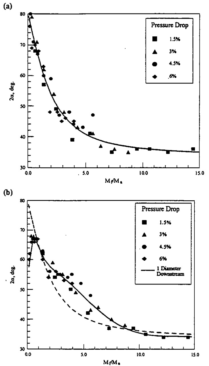
Figure 8. Spray angle measured downstream of the nozzle as a function of nozzle fuel/air momentum ratio and nozzle air pressure drop at 10 atm. air pressure: (a) one diameter, and (b) two diameters downstream of the nozzle.
