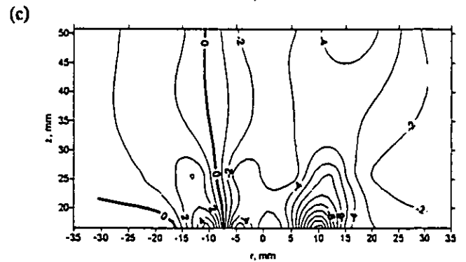
Figure 3. Pure Air-Blast Velocity (PAB) Contours (m/s): (a) axial, (b) azimuthal, and (c) radial.
