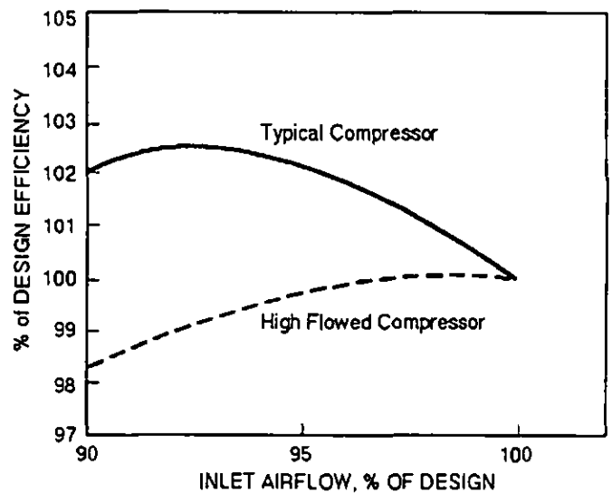
FIG. 7 - COMPARISON OF COMPRESSOR OPERATING LINE EFFICIENCY
