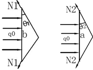
Fig. 8 Force equilibrium for the cross section of a plate
