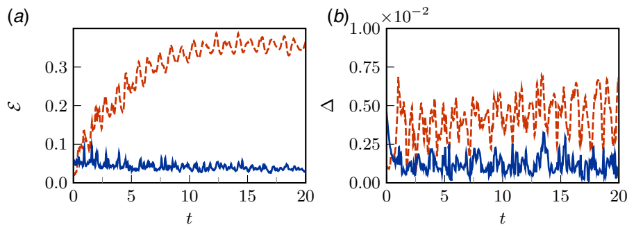
Fig. 3 Error ( N = 80 , \text{DOF} = 19 ); solid curves represent the reduced isolated system ( M = 10 ), short-dashed curve represents Galerkin reduction: (a) modal energy error and (b) displacement error in the interior region; \Delta \equiv \|\mathbf{x}_{\text{exact}} - \mathbf{x}_{\text{reduced}}\|_{s \in (0.25, 0.35)}
