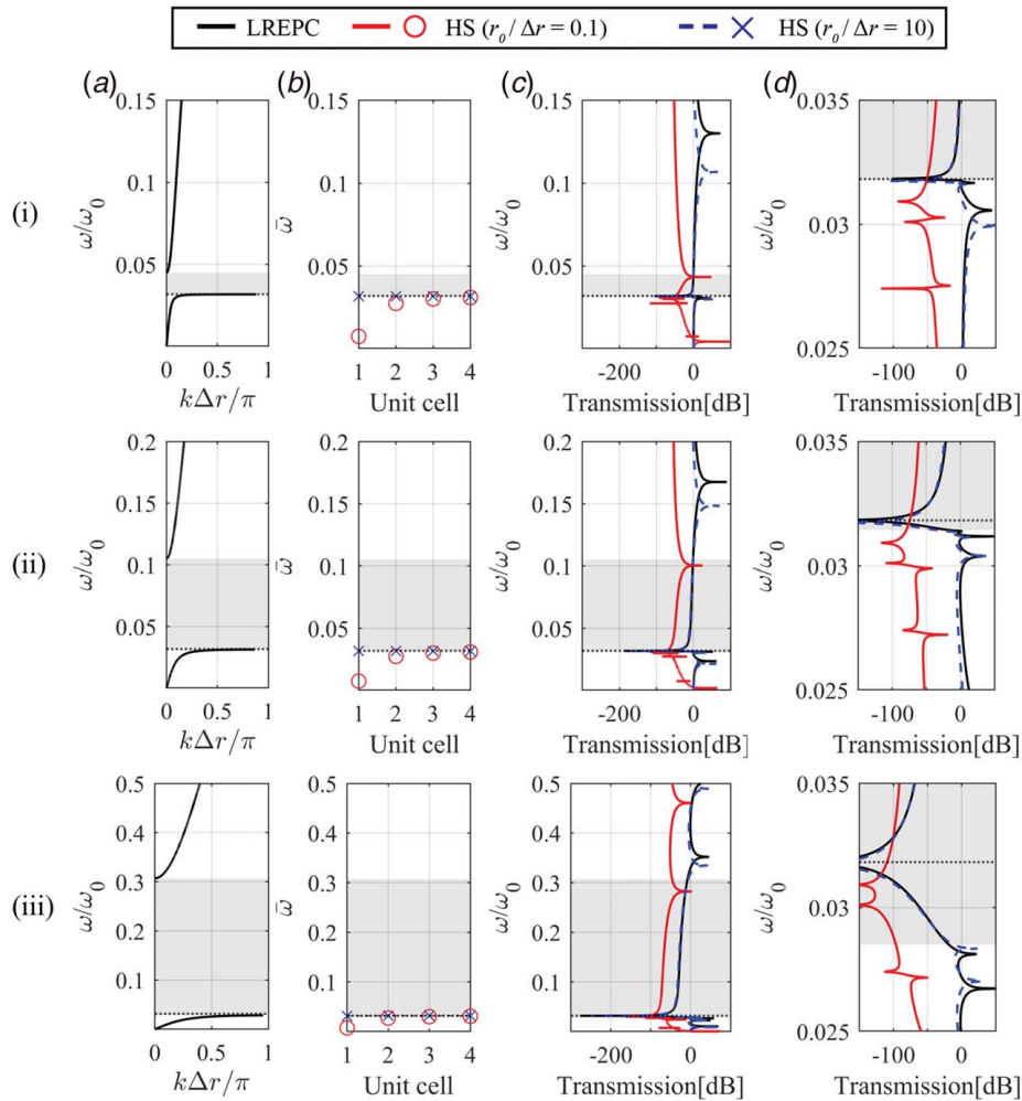
Fig. 2 (a) LREPC band structure, (b) dependence of \bar{\omega} on unit cell, (c) transmission, and (d) zoom in of transmission close to the lower band gap edge of the LREPC. Parameters for each row are as follows: (i) \bar{\beta}_{\text{LREPC}} = \bar{\beta}_{\text{HS}} = 0.01 and \bar{I}_{\text{LREPC}} = \bar{I}_{\text{HS}} = 1 , (ii) \bar{\beta}_{\text{LREPC}} = \bar{\beta}_{\text{HS}} = 0.1 and \bar{I}_{\text{LREPC}} = \bar{I}_{\text{HS}} = 10 , and (iii) \bar{\beta}_{\text{LREPC}} = \bar{\beta}_{\text{HS}} = 1 and \bar{I}_{\text{LREPC}} = \bar{I}_{\text{HS}} = 100 . Black-dotted lines indicate the resonance frequency of the LREPC resonators.
