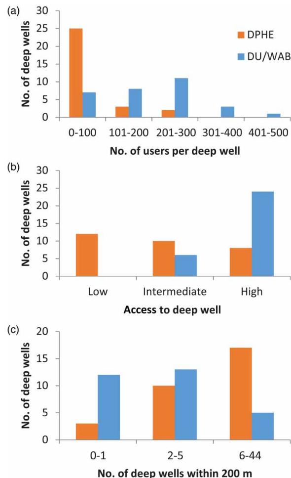
Figure 3 | Histogram of (a) the number of users per well, (b) the level of access to each deep well, and (c) the number of deep wells within 200 m of each deep well based on a survey of 30 randomly selected wells installed by DPHE and another 30 randomly selected wells installed by DU/WAB.
