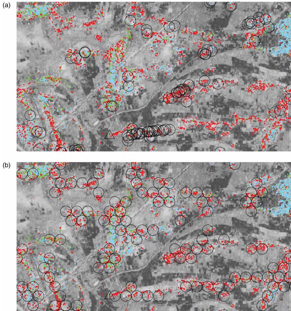
Figure 2 | Close-up map of a portion of Araihasar upazila with a high-resolution IKONOS image in grey-scale showing the status of wells with respect to As using the same symbols and color scale as in Figure 1: (a) the location of a subset of deep (>90 m) wells surveyed in 2012–13 and (b) the optimized location of a subset of the same number of wells selected from a regularly spaced grid. The two villages of Roynadi and Roynadi Kalagachhia contain four deep wells with >50 µg/L As that do not show evidence of a leak and are shown as larger circles. Please refer to the online version of this paper to see this figure in colour.
