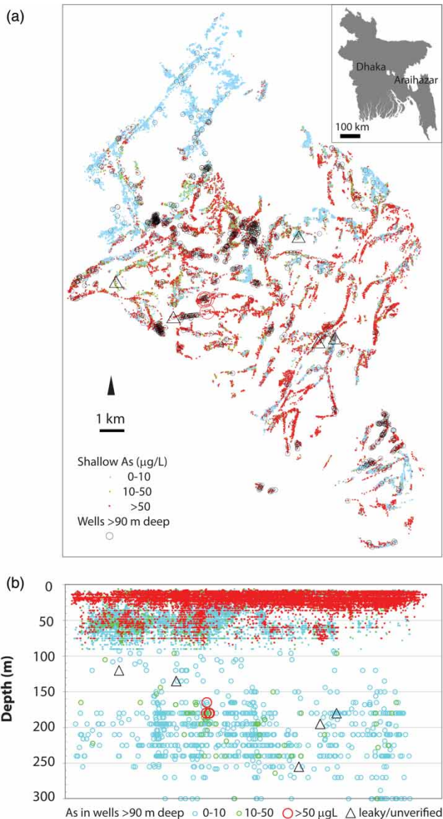
Figure 1 | (a) Map of Araihaazar upazila with colored dots used to show the status of 48,790 wells tested with a field-kit in 2012–13 with respect to As. The inset shows in white the area covered by Metropolitan Dhaka and Araihaazar within a map of Bangladesh. Shown as thin black circles with a radius of 100 m are the locations of 915 intermediate and deep (>90 m) wells. Black triangles indicate the location and depth of five deep wells with >50 µg/L As with leaky casings. Larger circles identify the location and four wells with >50 µg/L As that showed no indication of a shallow leak. (b) East-west depth section of the same data showing, in addition, the As content of deep wells according to the same color scale. Please refer to the online version of this paper to see this figure in colour.
