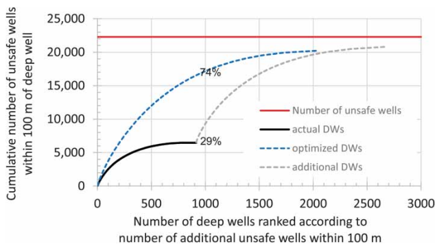
Figure 4 | Spatial calculation of the number of unsafe wells in Araihasar located within 100 m of deep wells according to three different scenarios. (a) The actual location of up to 915 deep wells surveyed in 2012–13. Each unsafe well is counted only once by assigning to the closest deep well, even if circles with a 100 m radius of existing deep wells overlap. (b) The hypothetical location of deep wells positioned on a regular grid and ranked according to the number of unsafe wells within 100 m. (c) The actual location of 915 deep wells and additional deep wells positioned on a regular grid.
