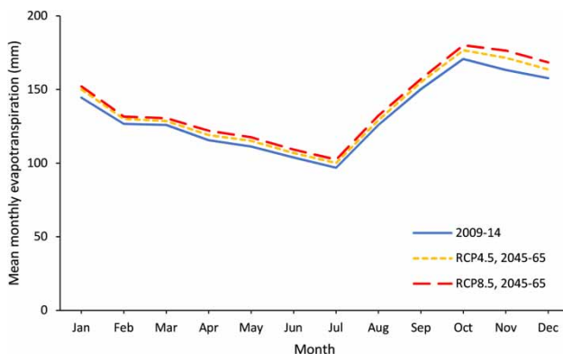
Figure 3 | Calculated monthly evapotranspiration for 2009–2014 and 2045–2065.
