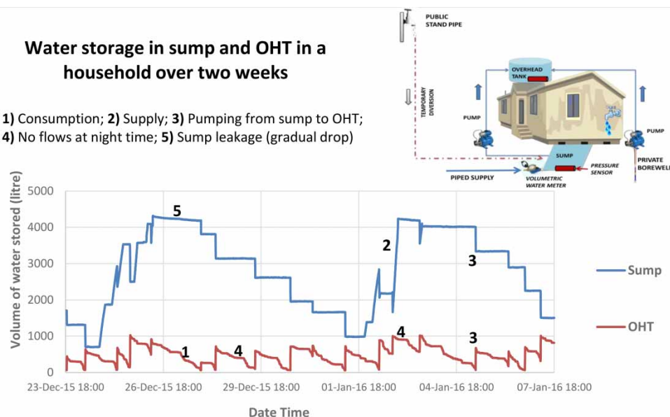
Figure 2 | Time series graph of water storage in a sump and OHT in a household.
