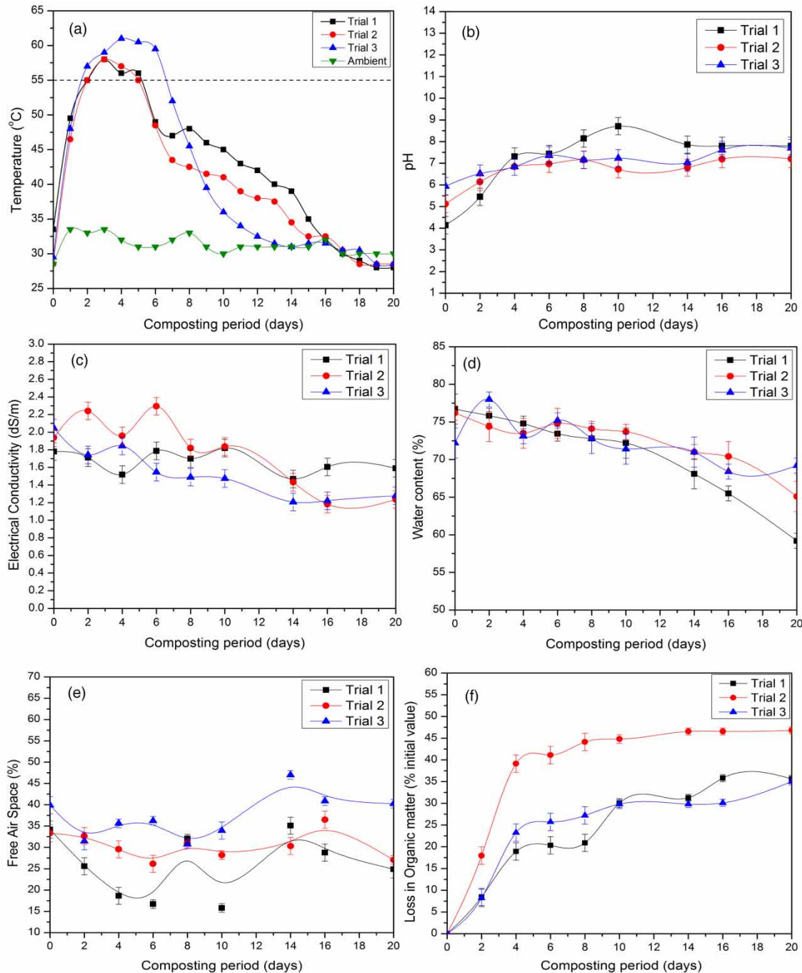
Figure 2 | Change in composting parameters: (a) temperature profile; (b) pH; (c) EC; (d) water content; (e) FAS; (f) loss of organic matter; (g) loss in total nitrogen; (h) ammonia-nitrogen; (i) nitrate-nitrogen; (j) total phosphorus; (k) potassium; (l) C/N ratio. (Continued.)
