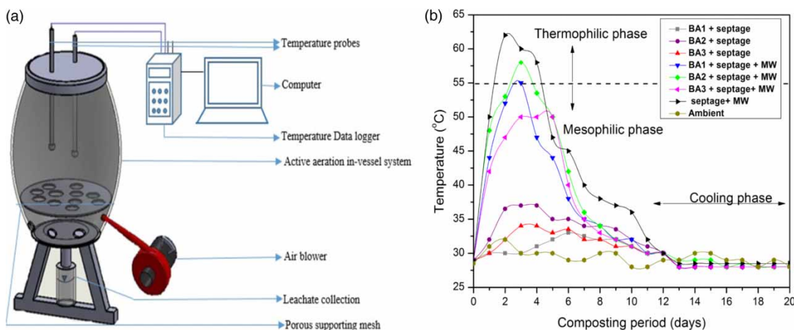
Figure 1 | (a) Experimental set-up of in-vessel co-composting system; (b) temperature profiles of trials with combination of various BAs, septage and MW. BA1: straw; BA2: coir pith; BA3: bagasse.
