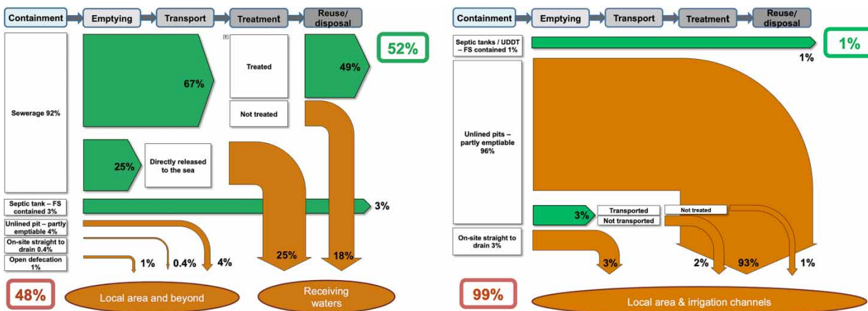
Figure 2 | SFDs for Lima, Peru showing contrasting results city-wide and for low-income settlements.
