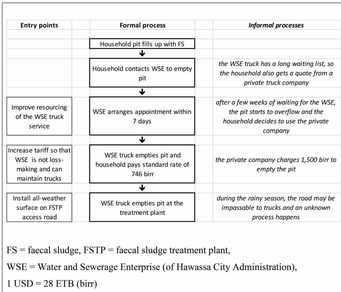
Figure 3 | Example of a process map: emptying a household latrine pit in Hawassa, Ethiopia.
