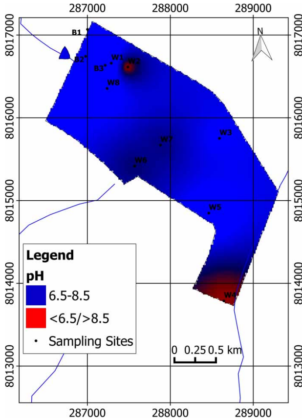
Figure 2 | Spatial distribution of pH for the period February to April 2015.
