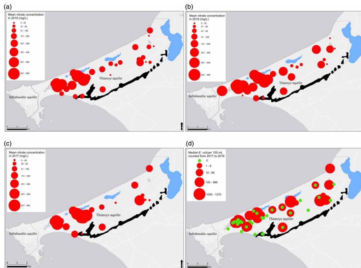
Figure 4 | Distribution of the mean nitrate concentrations (a – in 2019, b – in 2018, c – in 2017) and median E. coli counts (d – from 2017 to 2018) measured in the Thiaryoye shallow aquifer of Dakar.
