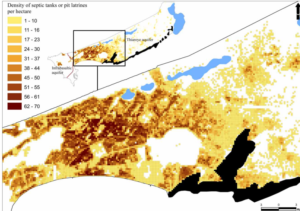
Figure 2 | Mapped density of on-site sanitation facilities (septic tanks, pit latrines) in the Thiaryoye shallow aquifer estimated from Quickbird satellite image (acquired on December 6, 2016) and field surveys (10–17 March 2018); inset map shows the broader geographical context from Figure 1.
