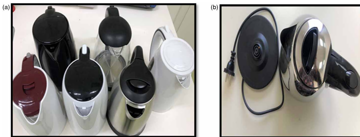
Figure 1 | (a) Various kettles used in the study and (b) kettle after dismantling.
