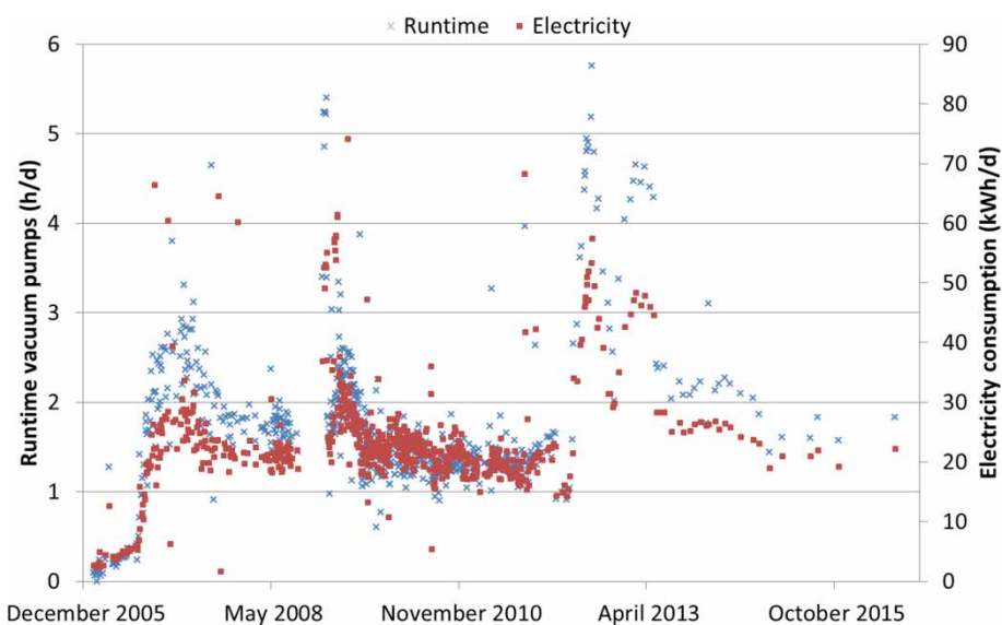
Figure 4 | Vacuum pump runtime (blue crosses) and electricity consumption (red dots) for the vacuum sewer system in Knittlingen, Germany.
