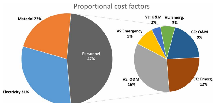
Figure 2 | Relative operational cost composition of vacuum sewers in Germany; VS: vacuum station; VL: vacuum lines; CC: collection chambers (average of 22 systems).
