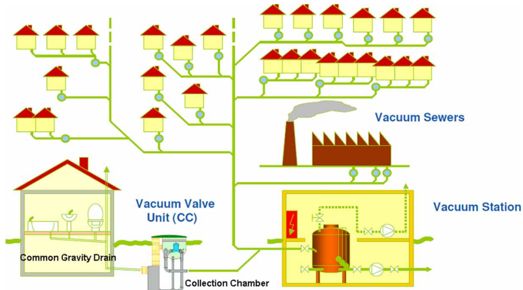
Figure 1 | Overview of a vacuum sewer system involving the vacuum valve unit at the valve pits, vacuum mains and the central vacuum station (Stauffer & Spuhler 2012).
