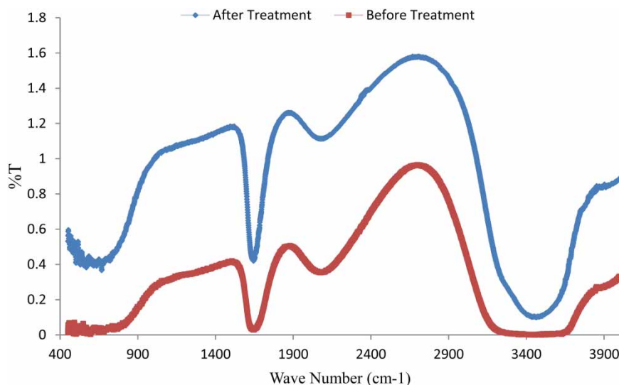
Figure 7 | Fourier Transformation Infrared Spectroscopy before and after treatment.
