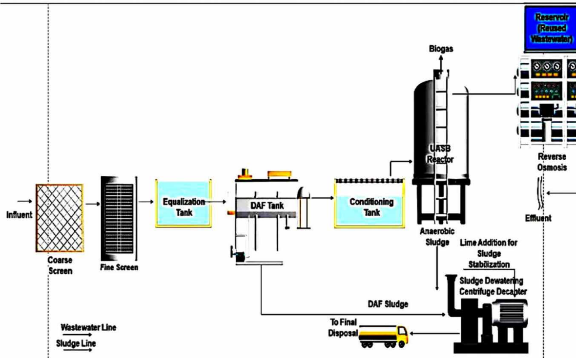
Figure 1 | Current wastewater treatment process flow diagram.
