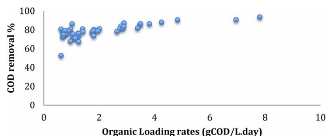
Figure 2 | tCOD removal efficiency in the SGBR with different OLR.
