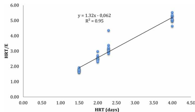
Figure 3 | Evaluation of Grau second-order model kinetic parameters.
