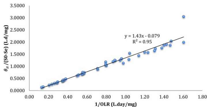
Figure 5 | Evaluation of modified Stover-Kincannon model kinetic parameters.
