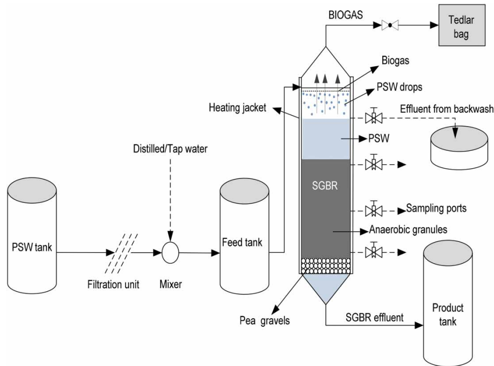
Figure 1 | Layout of the Static Granular Bed Reactor with basic parameters of the PSW used.
