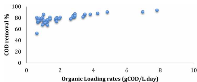
Figure 2 | tCOD removal efficiency in the SGBR with different OLR.
