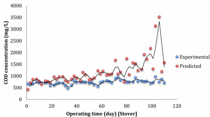
Figure 6 | Modified Stover-Kincannon model application.
