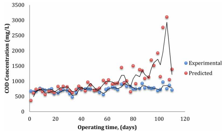
Figure 4 | Predicted and experimental COD concentration using Grau second order model.
