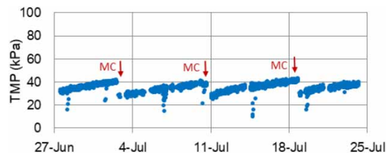
Figure 4 | TMP trend for the ceramic membrane train in CAWW.
