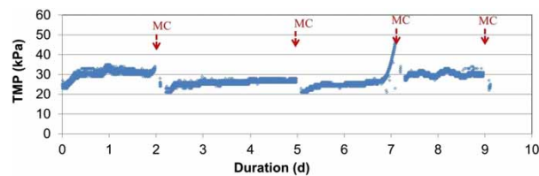
Figure 8 | TMP trend of run-C (249 LMH) in the seawater pretreatment pilot system.
