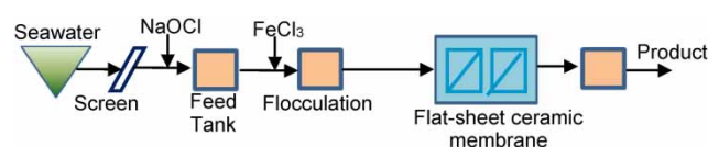
Figure 3 | Schematic diagram of the seawater pretreatment pilot system.
