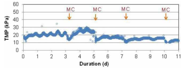
Figure 6 | TMP trend of run-A (181 LMH) in the seawater pretreatment pilot system.
