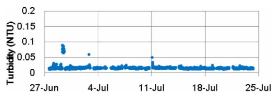
Figure 5 | Turbidity of permeate for the ceramic membrane train in CAWW.
