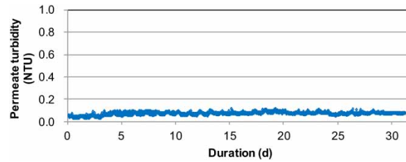
Figure 10 | Permeate turbidity during run-B condition in the seawater pretreatment pilot system.
