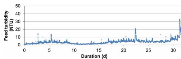
Figure 9 | Feed turbidity during run-B condition in the seawater pretreatment pilot system.
