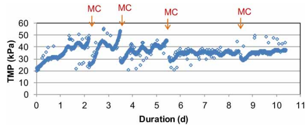
Figure 7 | TMP trend of run-B (218 LMH) in the seawater pretreatment pilot system.
