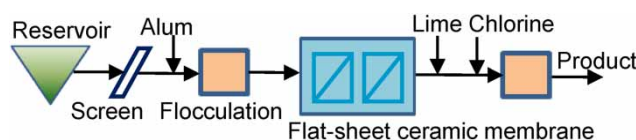
Figure 1 | Schematic flow diagram of water treatment in CAWW.
