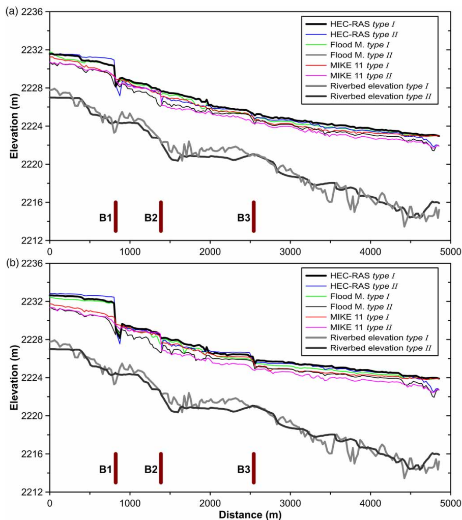
Figure 3 | Water surface elevations of two scenarios for three hydraulic models. (a) For a return period of 5 yr; (b) For a return period of 20 yr. B1, B2 and B3 show the location of bridges.
