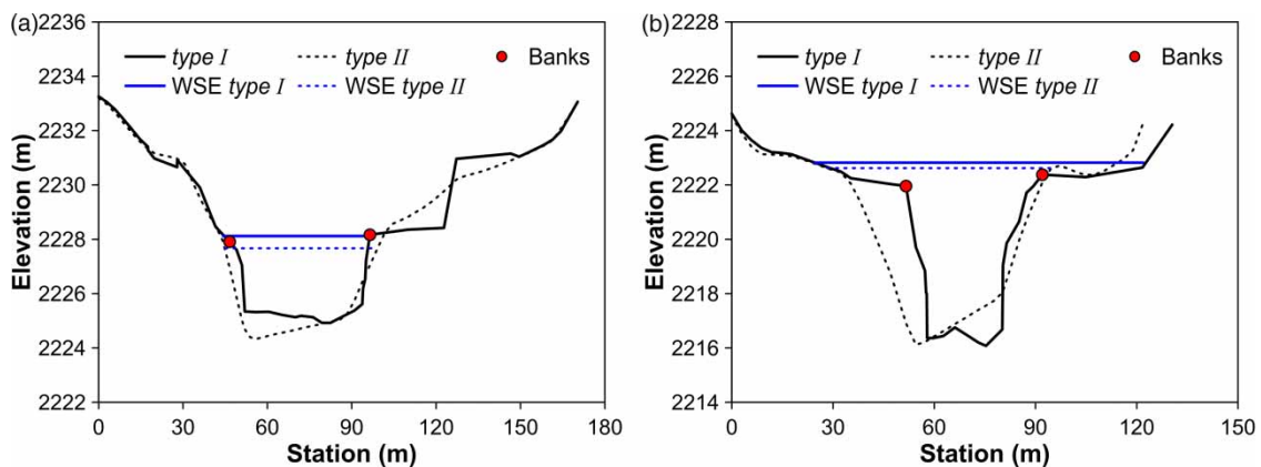
Figure 2 | Visual comparison of two cross sections located at 1,025.70 m (a) and 4,095.45 m (b) of the modeled river reach. Conventional topographic survey, using a total station, is represented by solid black lines ( type I data). Cross sections derived only from DEM information is represented by dotted lines ( type II data). The water surface elevation corresponding to the 2 yr return period is presented through the blue lines.
