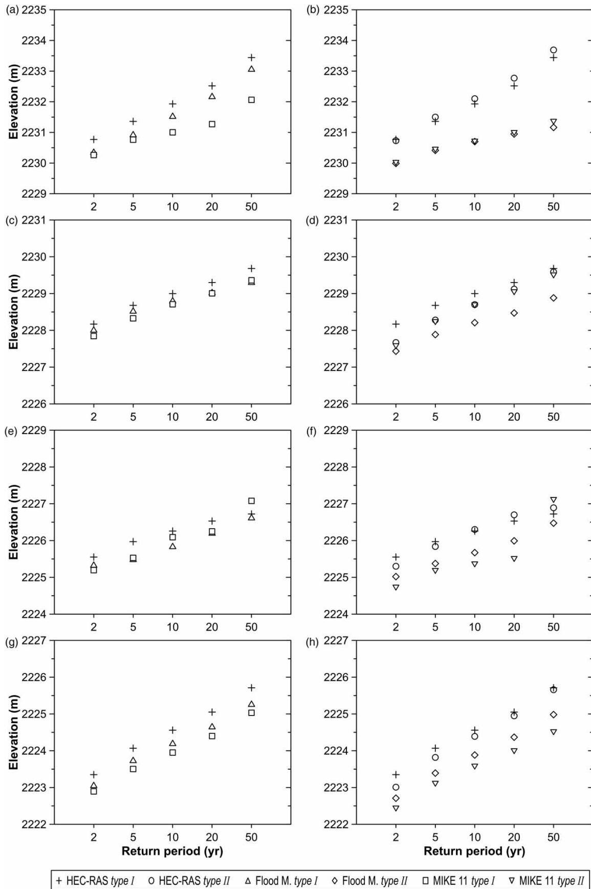
Figure 5 | Water surface elevations for different cross sections along the study transect. Left- type I and right- type II models correspondingly in each row. Distance in meters along river reach: (a-b) 315.33; (c-d) 1,025.70; (e-f) 2,109.19; (g-h) 3,689.93.
