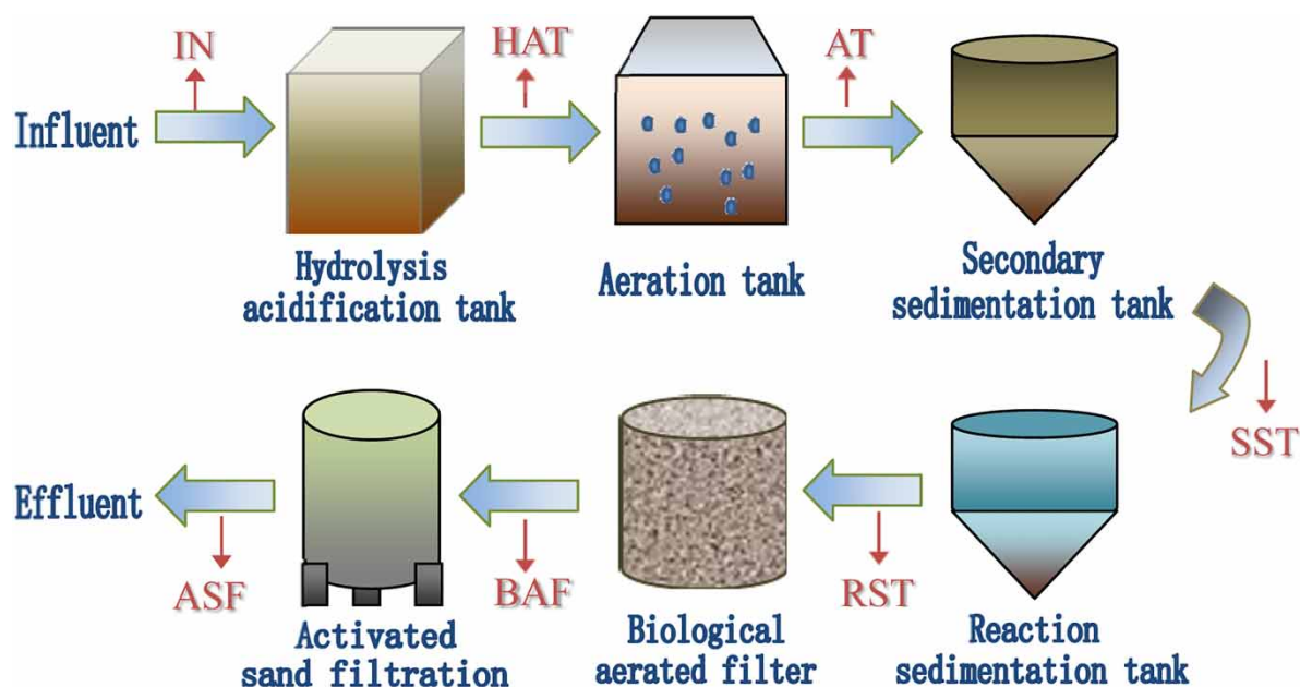
Figure 1 | Flow-process diagram for the industrial dye wastewater treatment (ID-WWTP).
