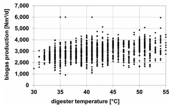
Figure 5 | Relationship between biogas production and temperature for #WWTP_A.
