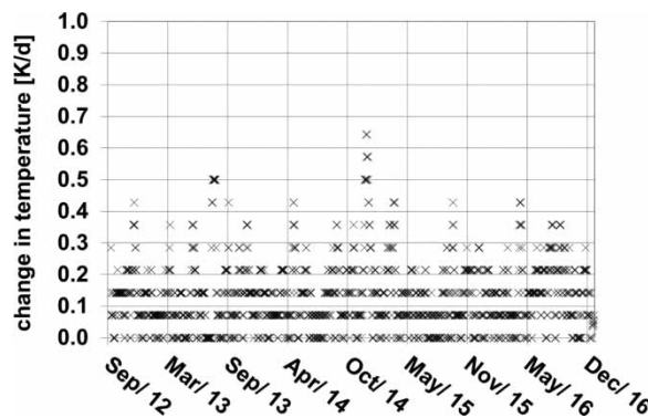
Figure 3 | Temperature change per day in #WWTP_A_D1.
