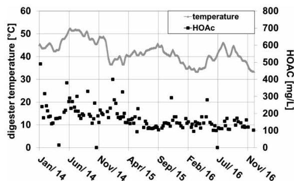
Figure 12 | Organic acid concentration in digester of #WWTP_A_D1.
