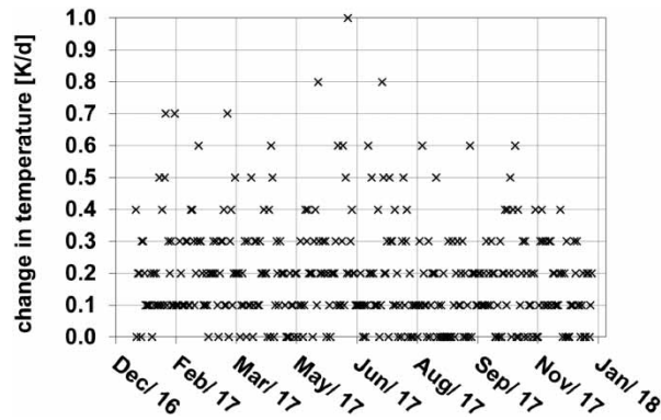
Figure 4 | Temperature change per day in #WWTP_B_D1.
