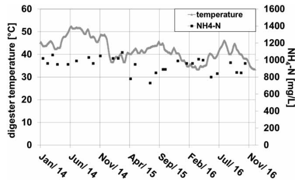
Figure 13 | Ammonium concentration in #WWTP_A_D1.
