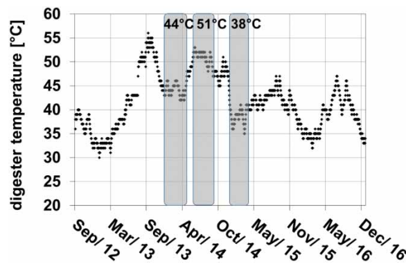
Figure 10 | Identified temperature ranges of #WWTP_A.
