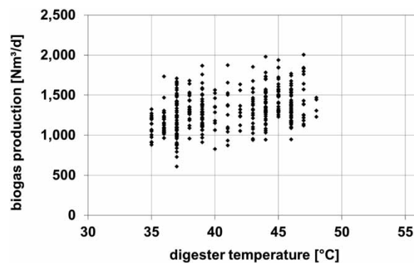
Figure 6 | Relationship between biogas production and temperature for #WWTP_B.
