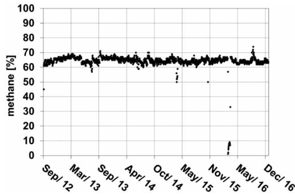
Figure 7 | Methane concentration of #WWTP_A.
