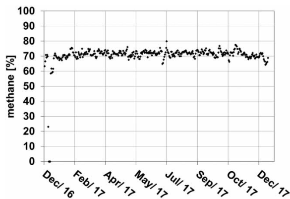
Figure 8 | Methane concentration of #WWTP_B.
