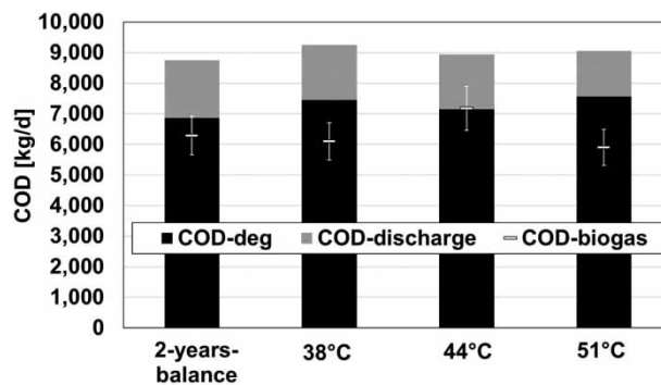
Figure 11 | Results of the COD balancing of the different periods #WWTP_A.
