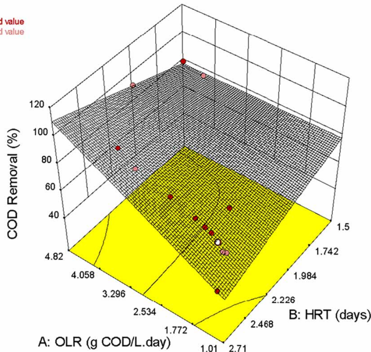
Figure 2 | 3D plot of OLR (A) and HRT (B), and their effect on EGSB's COD removal efficiency.
