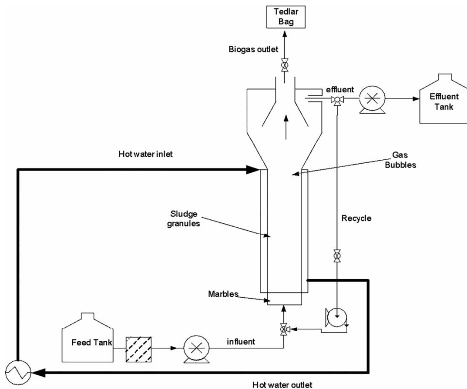
Figure 1 | Schematic illustration of the EGSB set-up treating PSW.
