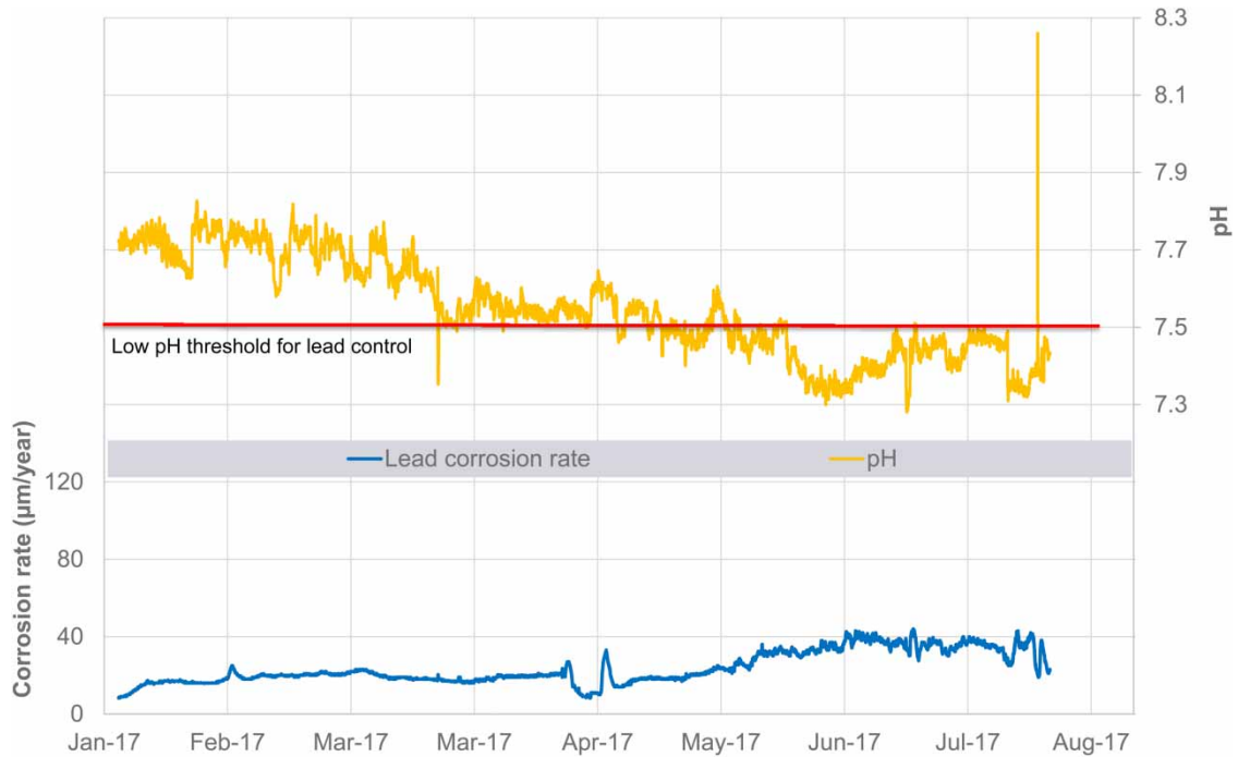
Figure 6 | Plant performance for monitoring and control of lead corrosion risk (via target pH set at >7.5).
