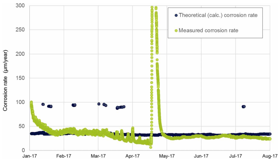
Figure 7 | Plant performance for monitoring and control of iron corrosion potential (via target corrosion rate set at <50 µm/year).
