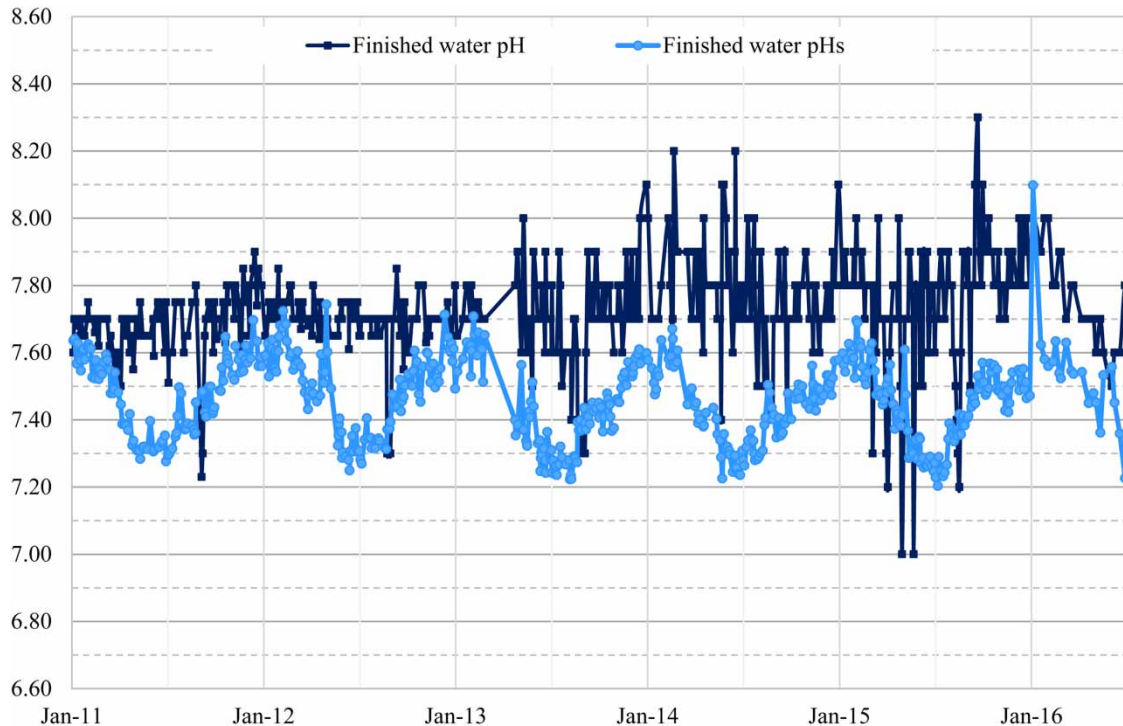
Figure 1 | Actual finished water pH and calculated values of the saturation pH over 2011–2016.
