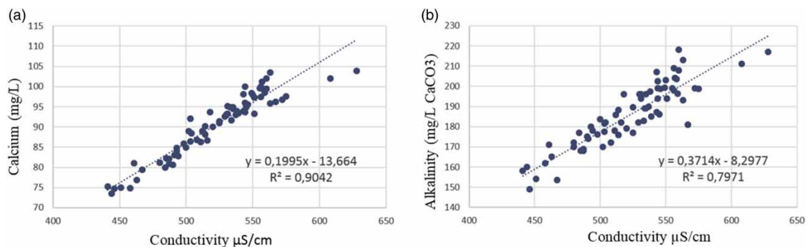
Figure 3 | Correlation between conductivity as online surrogate and (a) calcium and (b) alkalinity (2011–2016 data).
