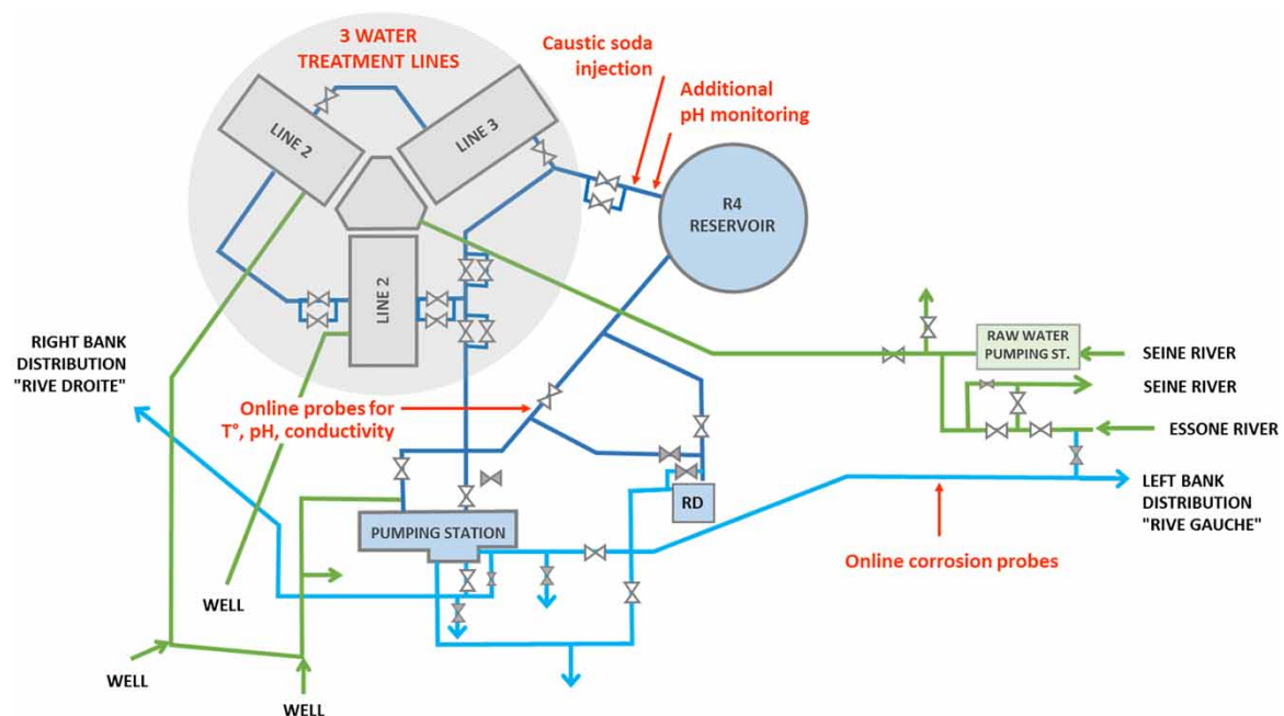
Figure 2 | Plant schematic with corrosion control system.
