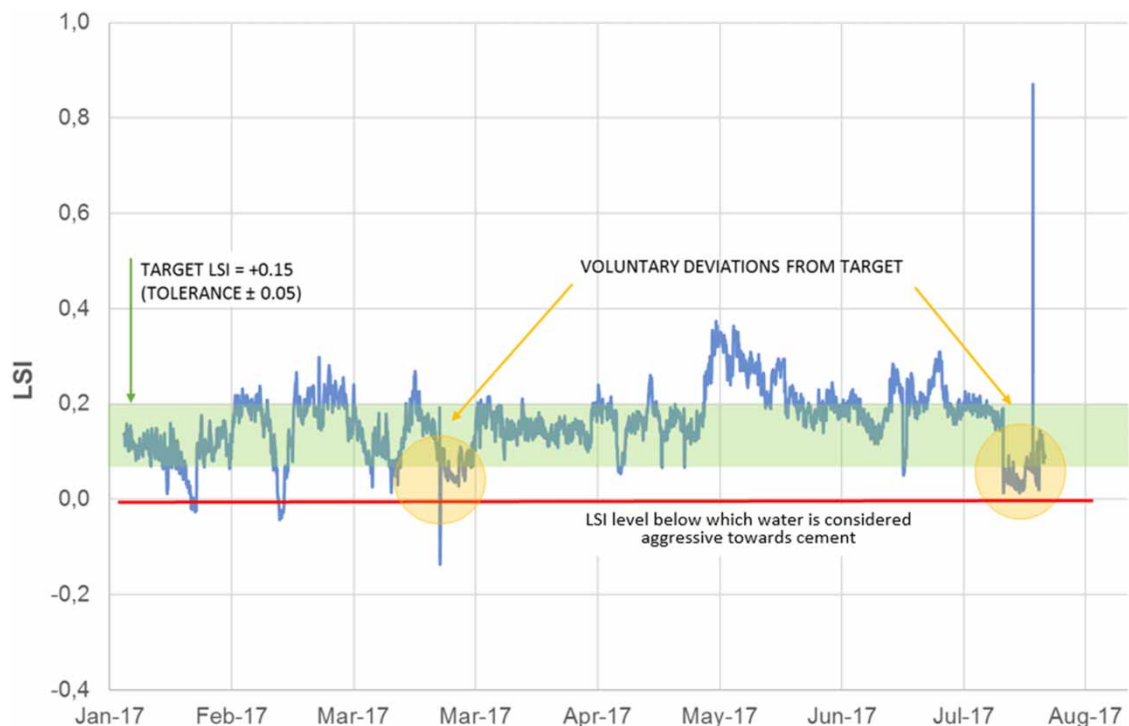
Figure 5 | Plant performance for monitoring and control of cement corrosion potential (via target LSI of 0.15 \pm 0.05 ).
