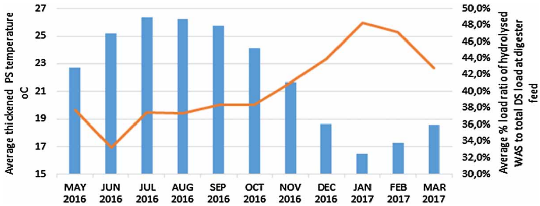
Figure 4 | DS load ratio of hydrolysed WAS to total DS load at digester feed and thickened PS stream temperature.
