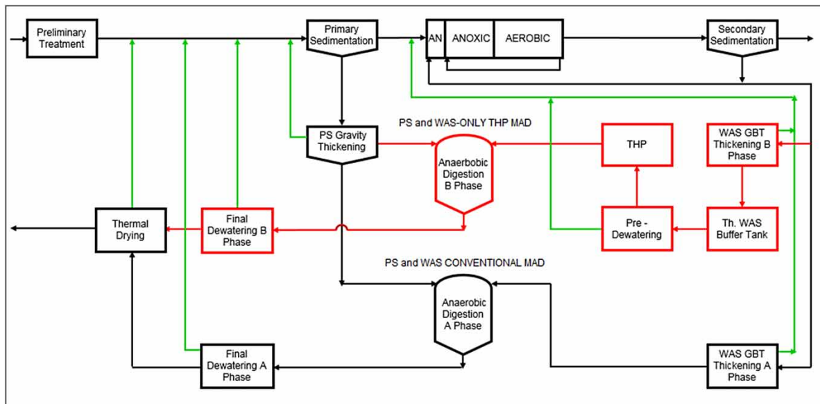
Figure 2 | Simplified flow diagram of the wastewater and sludge treatment lines of Psytalia WWTP. The WAS-only treatment sludge line is highlighted in red.
