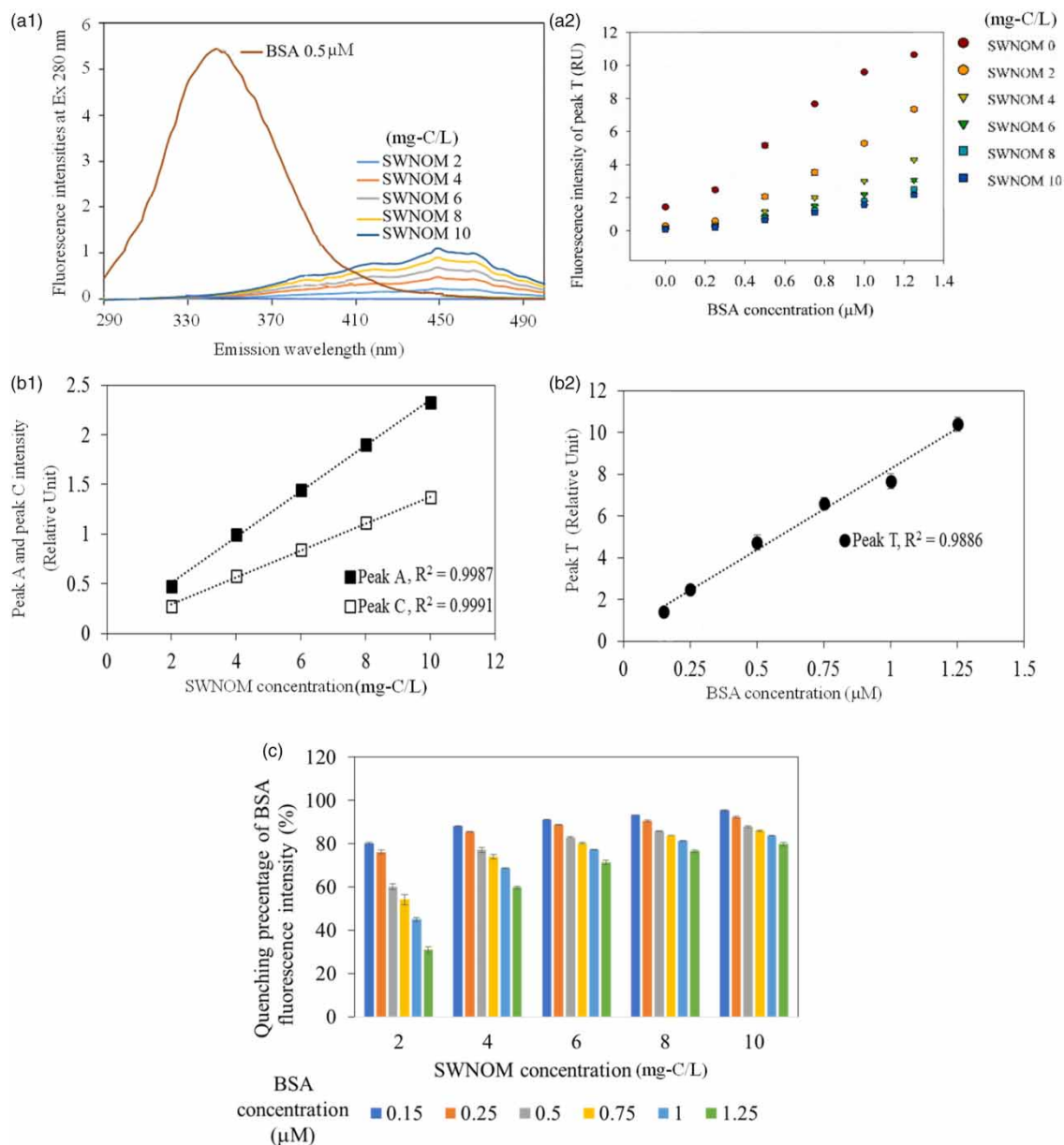
Figure 2 | (a1) Overlapping fluorescence spectrum of SWNOM and BSA, (a2) fluorescence peak intensity of BSA in the presence of varying concentrations of SWNOM; (b) relationship between fluorescence peak intensity and varying concentrations of (b1) SWNOM, and (b2) BSA. (c) Quenching percentage of BSA fluorescence intensity at different concentrations of BSA and SWNOM.
