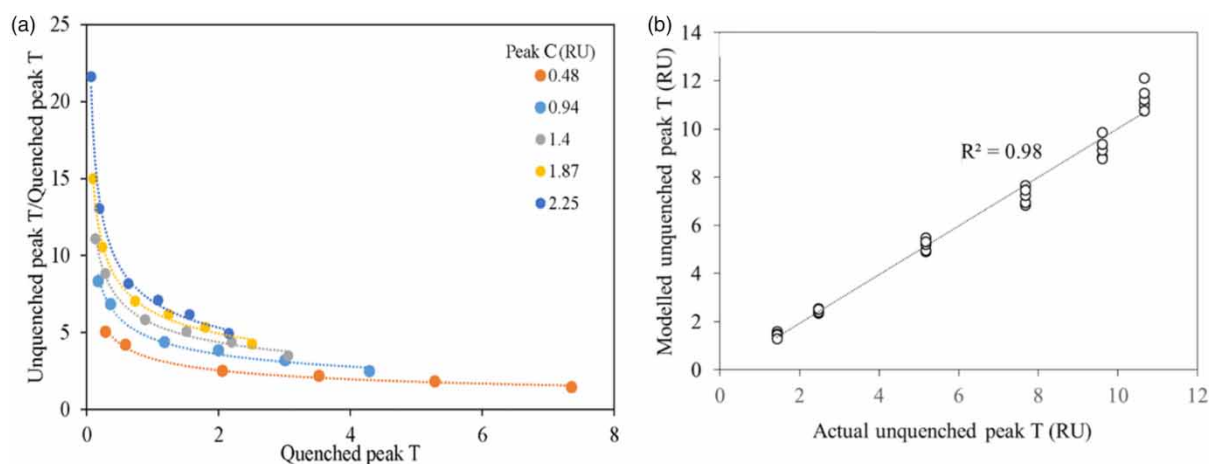
Figure 4 | (a) Relationship between unquenched peak T/quenched peak T vs. quenched peak at different peak C levels, (b) modelled vs. actual unquenched peak T fluorescence intensity.
