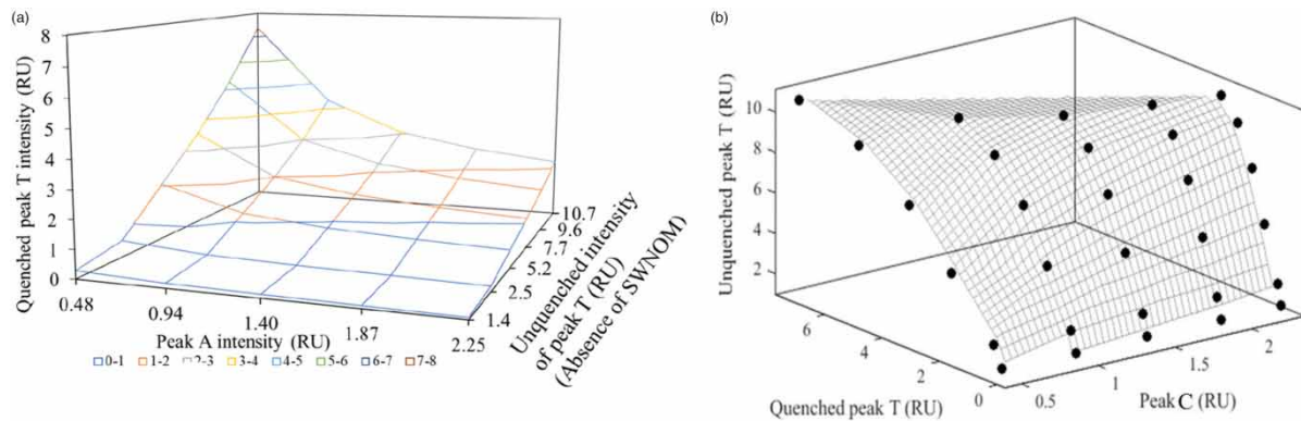
Figure 3 | (a) Effect of BSA and SWNOM concentration on peak T's quenched intensity. BSA concentration presented in terms of peak T's unquenched intensity, T (RU); SWNOM concentration in terms of peak C (RU). (b) Relationship between BSA's unquenched peak T and its quenched peak T and peak C (the grid pane is for visualization of the data pattern).
