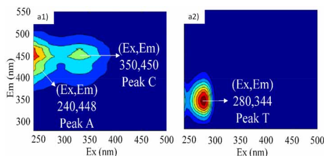
Figure 1 | PARAFAC components of fluorescence titration between – (a1) BSA and SWNOM (peaks A and C); and (a2) fluorescence intensity of BSA only (in the absence of SWNOM) (peak T).
