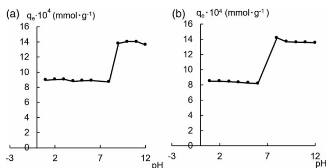
Figure 1 | Effect of pH on MB adsorption on (a) – RH-1, (b) – RH-2.
