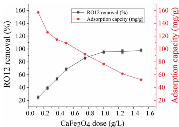
Figure 5 | The effect of CaFe 2 O 4 nanoparticles dose on RO12 removal (%) and adsorption capacity (mg/g).
