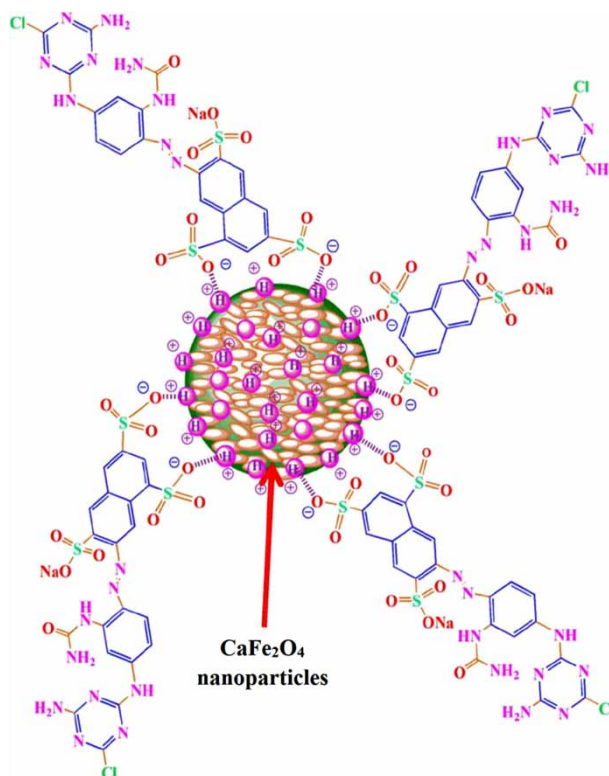
Figure 4 | Schematic illustration of electrostatic interaction between protonated CaFe 2 O 4 nanoparticle surface and anionic RO12 dye species.
