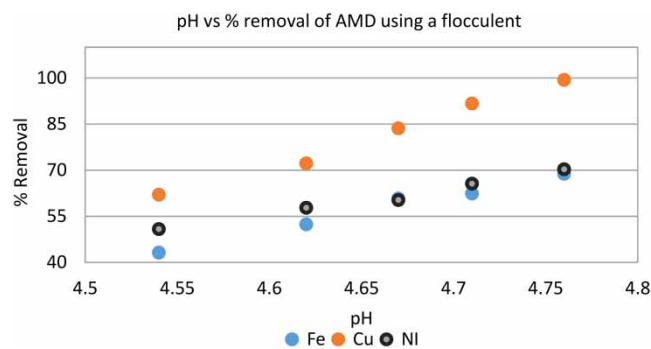
Figure 5 | pH vs % removal of Fe, Cu and Ni from AMD using flocculent 1.
