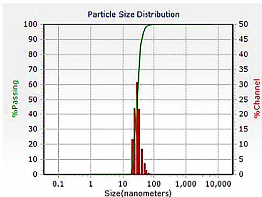
Figure 4 | Dynamic Light Scattering (DLS) images of the grown MWCNT/ ZrO_2 nanostructures via hydrothermal method with different growth temperatures.
