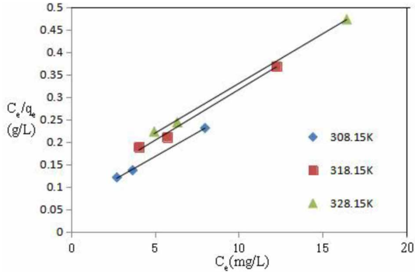
Figure 7 | Langmuir adsorption isotherm (adsorbent dosage: 1.67 g/L, pH: 9.5).
