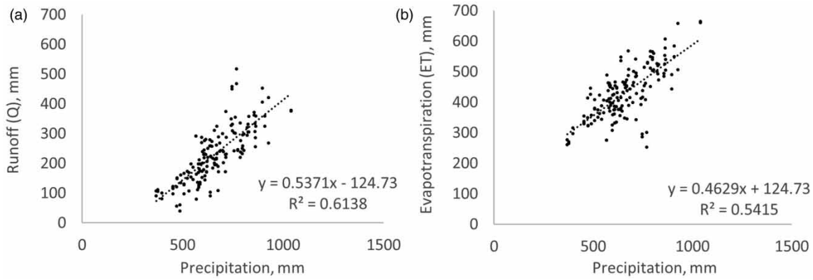
Figure 2 | The effect of yearly precipitation on water balance components in Berze, Mellupite and Vienziemite from 1995 until 2019.
