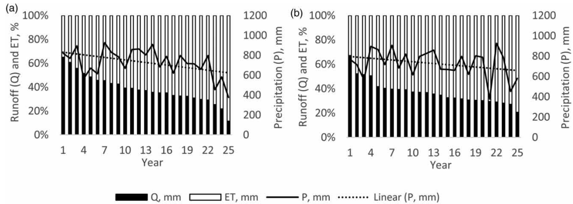
Figure 5 | The precipitation impact on water balance in Vienziemite from 1995 until 2019 sorted descending according to runoff contribution: (a) small catchment; (b) drainage field.
