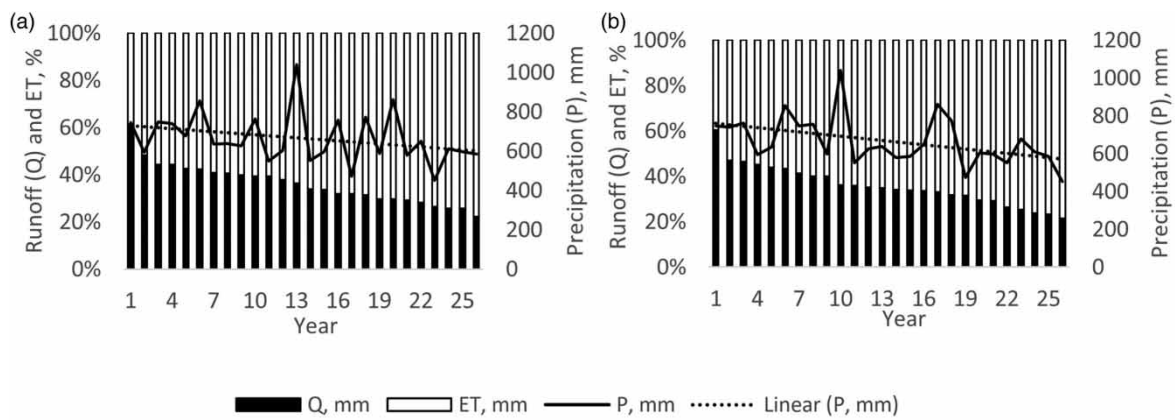
Figure 3 | The precipitation impact on water balance in Mellupite from 1995 until 2019 sorted descending according to runoff contribution: (a) small catchment; (b) drainage field.
