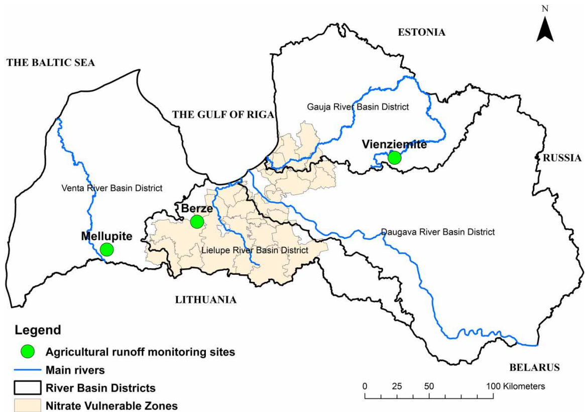
Figure 1 | Location of the agricultural monitoring sites of Berze, Mellupite, and Vienziemite.
