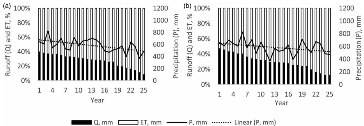
Figure 4 | The precipitation impact on water balance in Berze from 1995 until 2019 sorted descending according to runoff contribution: (a) small catchment; (b) drainage field.
