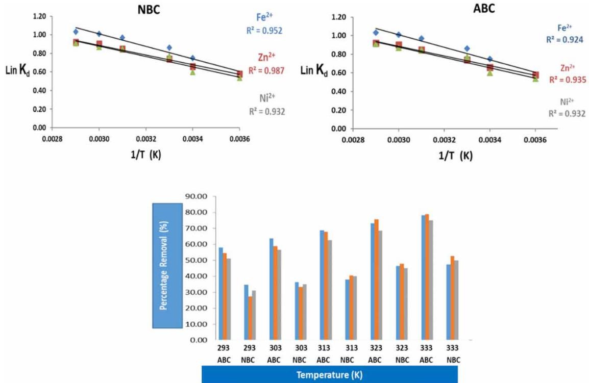
Figure 7 | Van't Hoff plots for Fe 2+ , Zn 2+ and Ni 2+ adsorption onto NBC and ABC at 293, 303, 313, 323 and 333 K.
