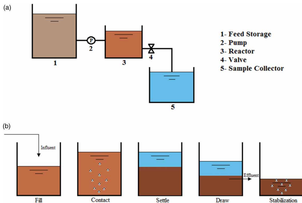
Figure 1 | (a) Schematic diagram of the experimental system, (b) Processes in the contact stabilization reactor.
