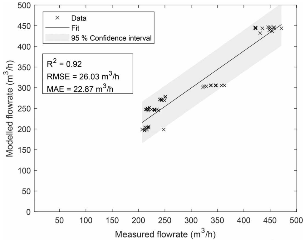
Figure 5 | The measured and modelled wastewater flowrates ( \text{m}^3/\text{h} ) with a linear fit line, the 95% confidence interval, and the performance values of the developed model using all the training data (58 data points) collected during the manual field measurement campaign.
