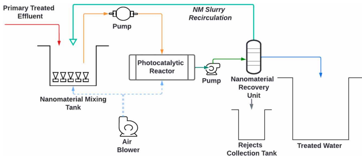
Figure 2 | Process flow diagram of the heterogeneous photocatalysis system based on TERI Advanced Oxidation Technology (TADOX ® ) (Bahadur & Bhargava 2019; Bahadur et al. 2023b).
