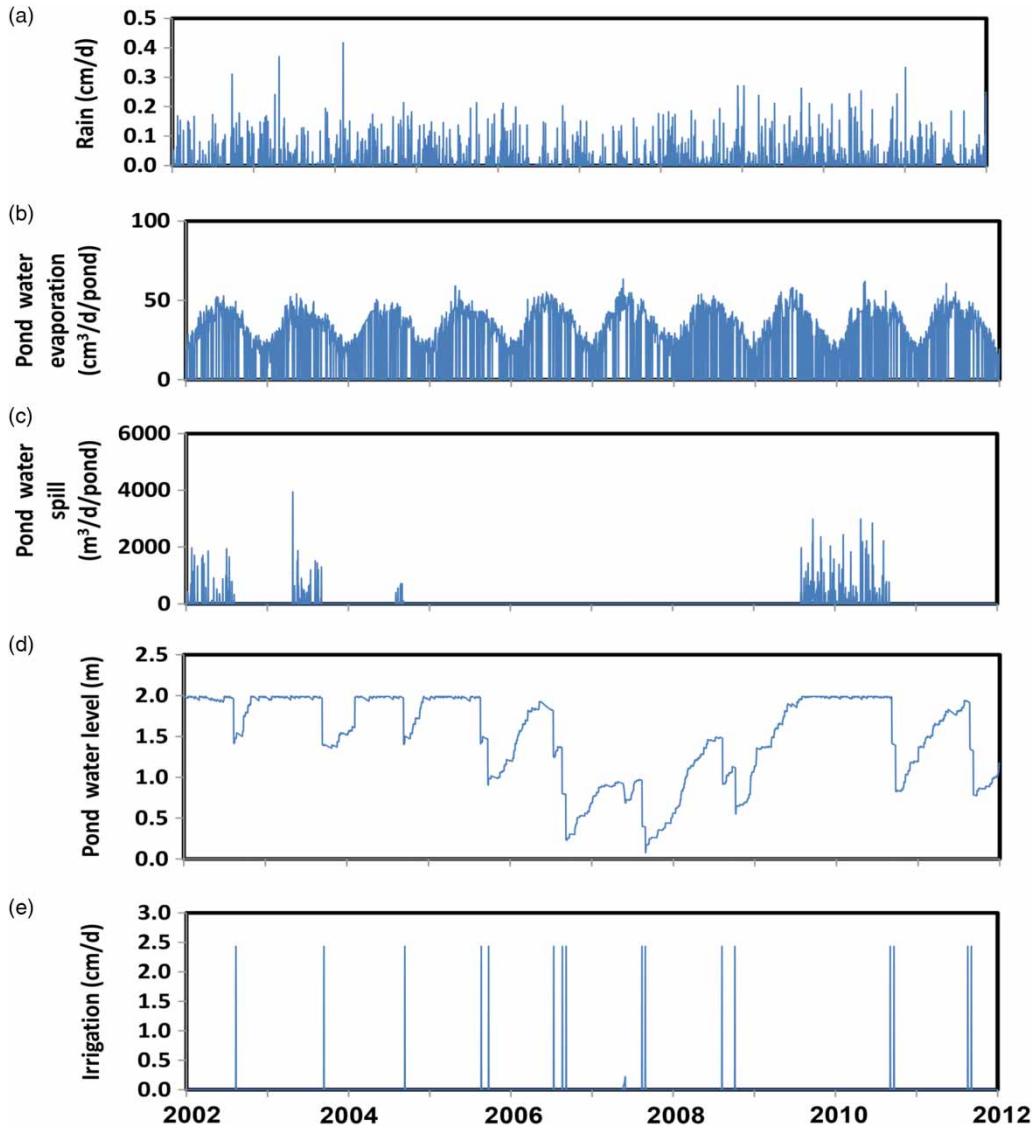
Figure 4 | Annual variations of daily rainfall (a), pond evaporation (b), pond spill (c), pond level (d), and irrigation rate (e) during a 10-year simulation from 2002 to 2012 for conditions with using pond water for soybeans irrigation.
