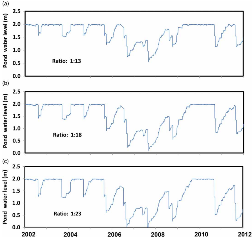
Figure 5 | Comparison of pond water levels among ratios of pond size to soybeans irrigation land areas: 1:13 (a), 1:18 (b), and 1:23 (c) during a 10-year simulation from 2002 to 2012.
