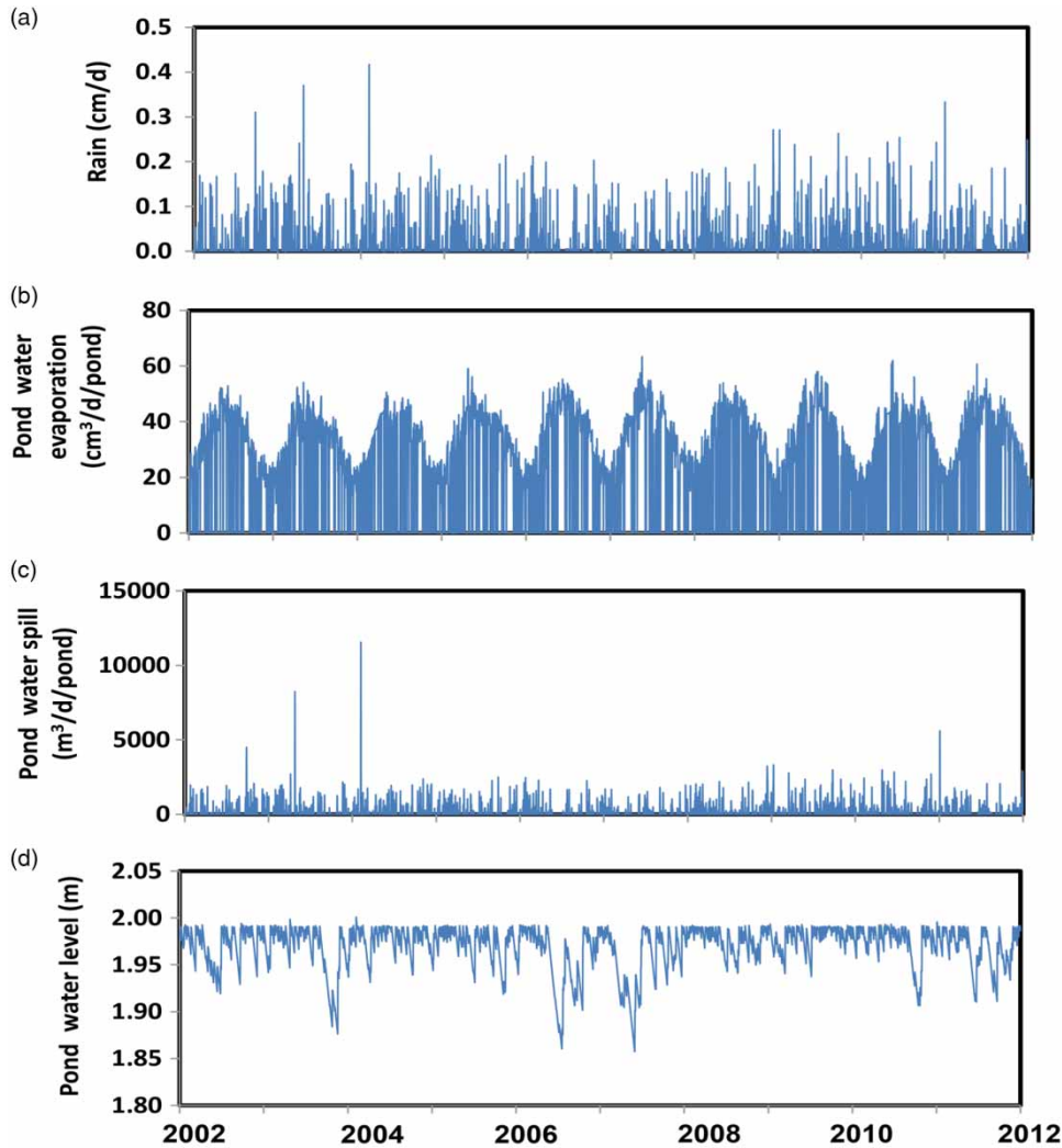
Figure 3 | Annual variations of daily rainfall (a), pond evaporation (b), pond spill (c), and pond level (d) during a 10-year simulation from 2002 to 2012 for conditions without using pond water for soybeans irrigation.
