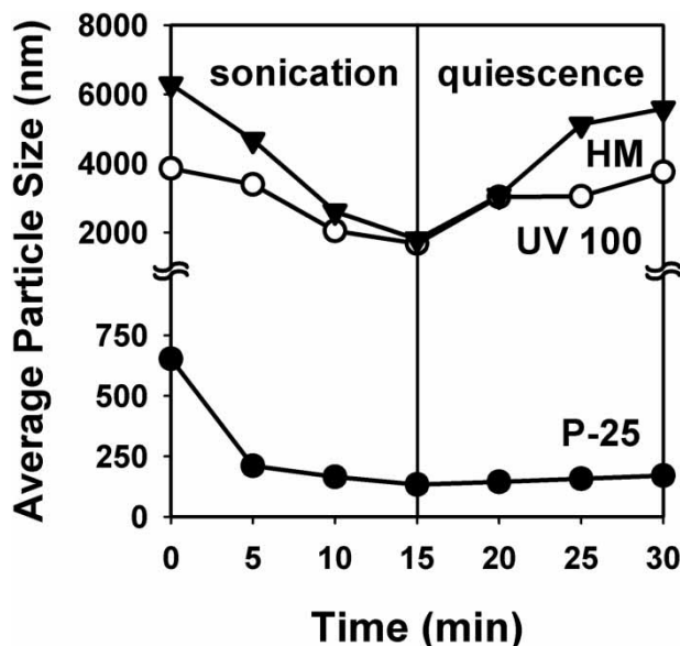
Figure 2 | Colloidal response of P-25, UV 100, and HM TiO 2 particles to sonication (TiO 2 concentration: 50 mg/l; sonication intensity: 60 W; pH: 5.2–5.8 with no control).
