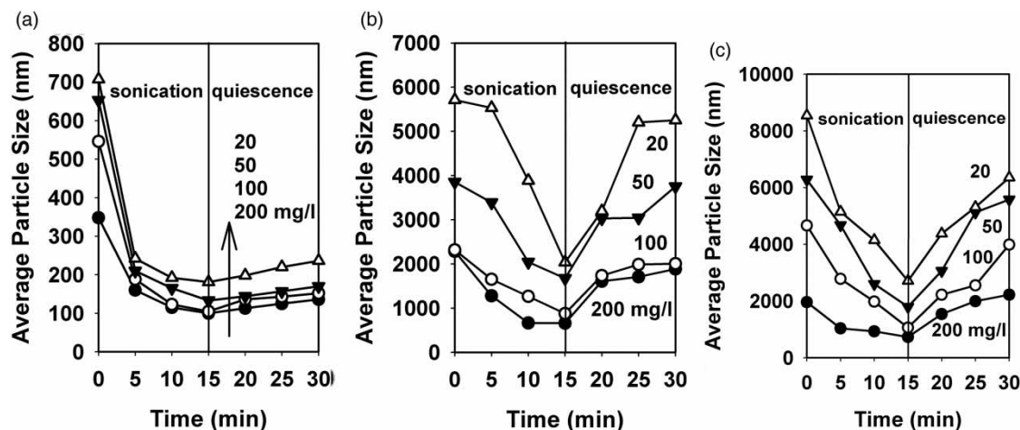
Figure 4 | Colloidal response of (a) P-25, (b) UV 100, and (c) HM TiO 2 particles at different concentrations of 20, 50, 100, and 200 mg/l to sonication (TiO 2 concentration: 20–200 mg/l; sonication intensity: 60 W; pH: 5.2–5.8 with no control).
