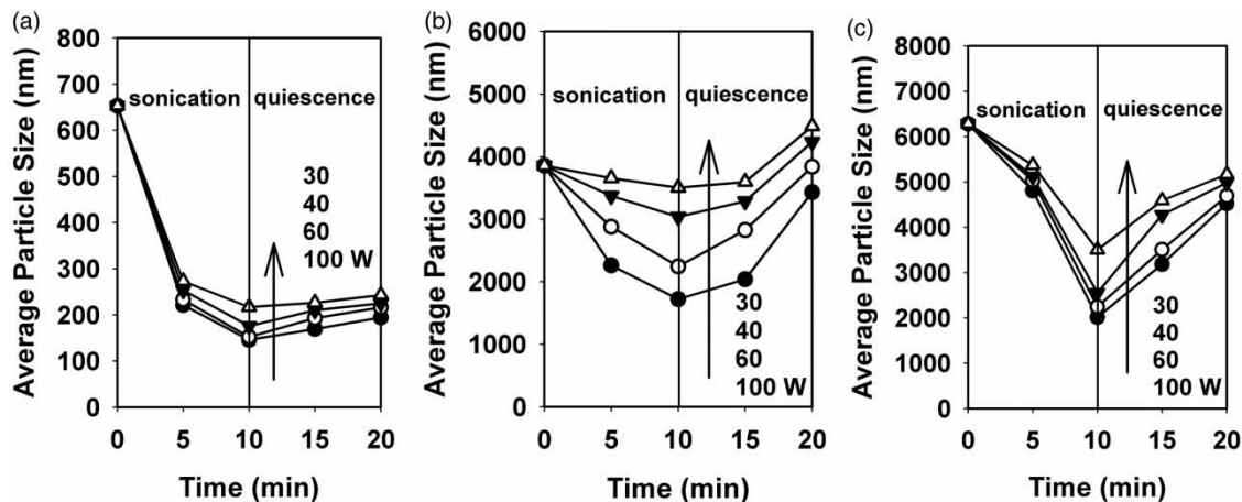
Figure 3 | Colloidal response of (a) P-25, (b) UV 100, and (c) HM TiO 2 particles to sonication at intensities of 30, 40, 60, and 100 W (TiO 2 concentration: 50 mg/l; sonication intensity: 30–100 W; pH: 5.2–5.8 with no control). It should be noted that 10 min were used in this specific study instead of 15 min because a combination of 15 min and 100 W greatly damaged the sonication probe.
