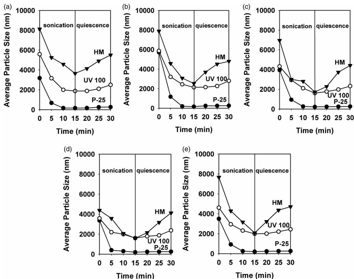
Figure 6 | Colloidal response of P-25, UV 100, and HM TiO 2 particles at different pHs of (a) 3, (b) 5, (c) 7, (d) 9, and (e) 11 to sonication (TiO 2 concentration: 50 mg/l; sonication intensity: 60 W; pH: 3–11).
