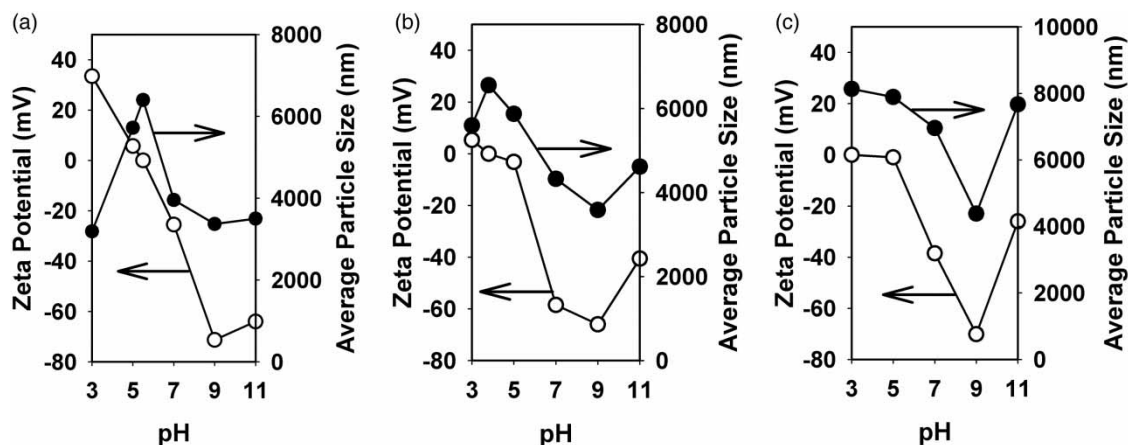
Figure 5 | Effect of solution pH on the size and zeta potential of TiO 2 particles: (a) P-25, (b) UV 100, and (c) HM. In each TiO 2 , pH PZC (pH where zeta potential is zero) can be determined.
