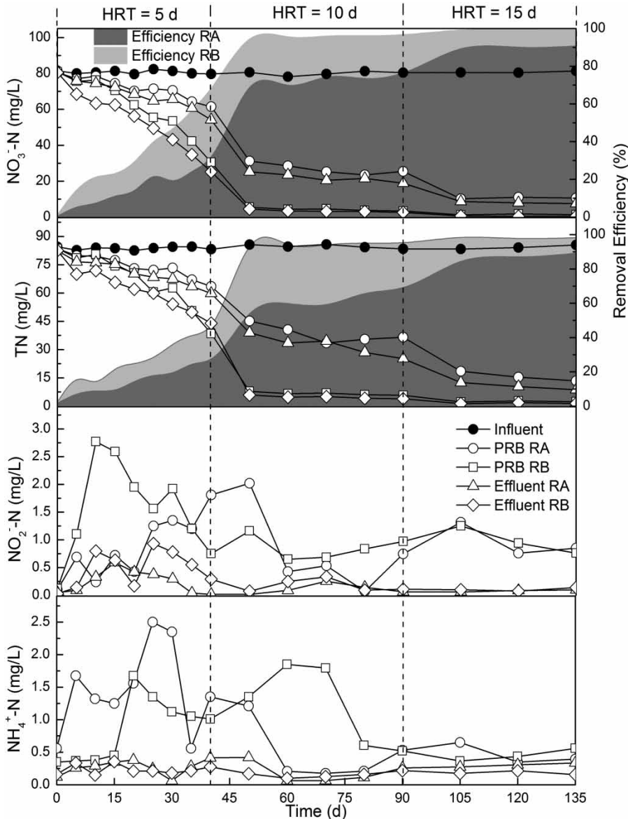
Figure 3 | Evolution of nitrate ( \text{NO}_3^- -N), total nitrogen (TN), nitrite ( \text{NO}_2^- -N), ammonium ( \text{NH}_4^+ -N) (mg/L), and removal efficiency (%) for in-situ dynamic groundwater remediation experiments.
