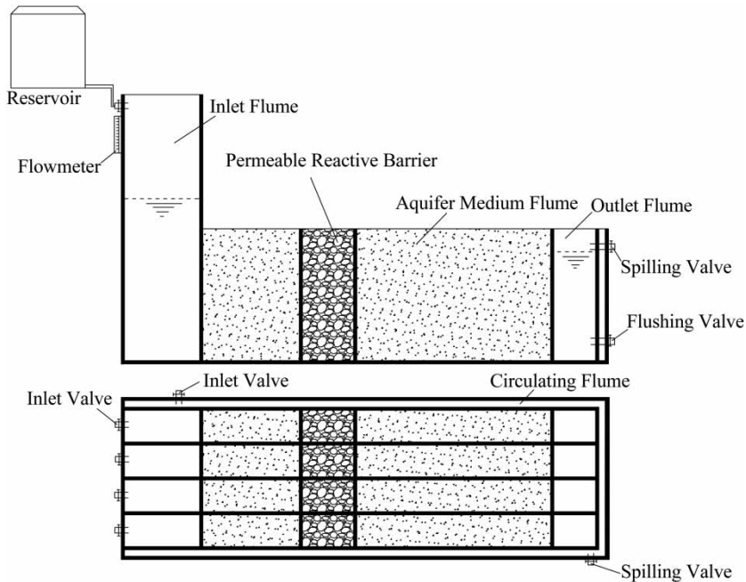
Figure 1 | Schematic of the in-situ remediation system.
