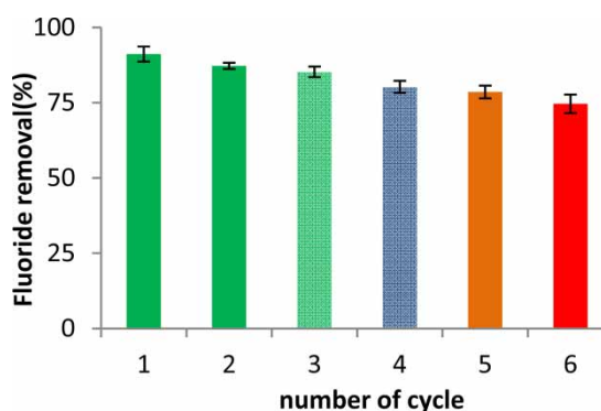
Figure 7 | Percentage of fluoride removal by the nanocomposite in different cycles.
