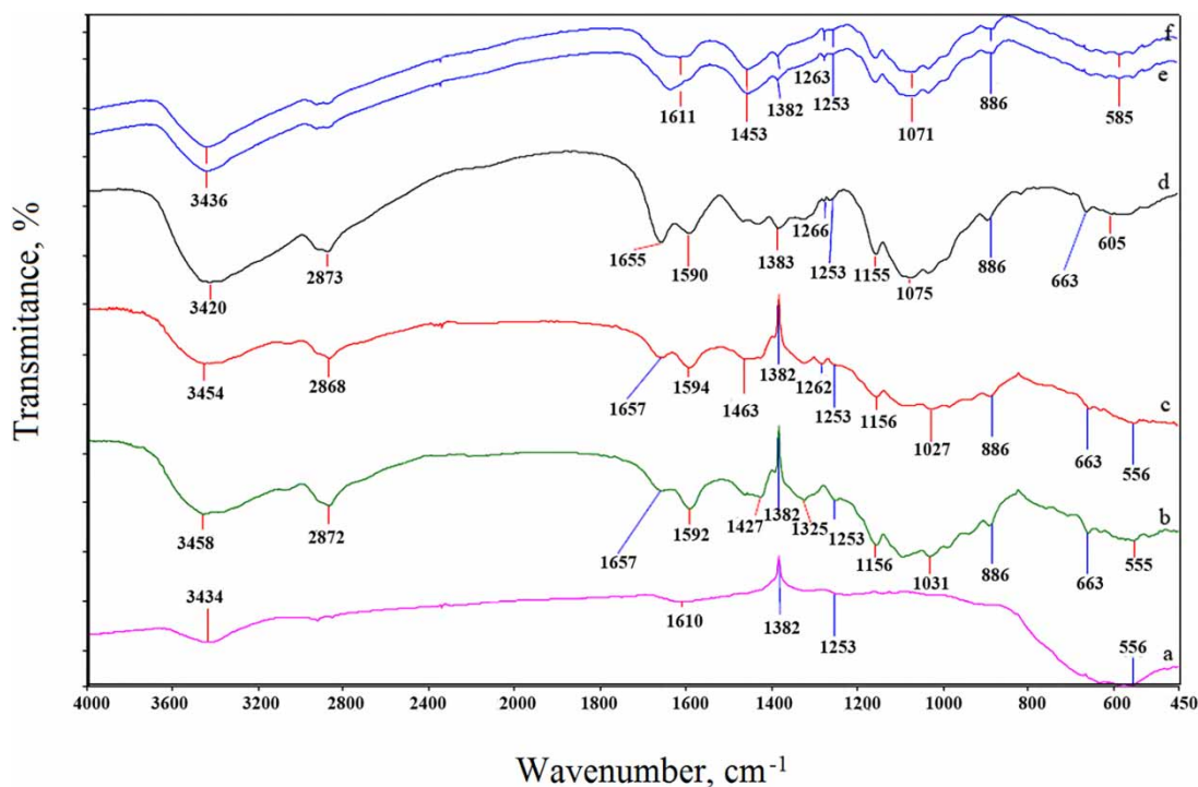
Figure 1 | FT-IR spectra of (a) \text{Fe}_3\text{O}_4@\text{TiO}_2 , (b) chitosan, (c) chitosan chloroacetyl chloride, (d) chitosan chloroacetyl chloride-2-(2-aminoethylamino)ethanol, (e) nanocomposite, (f) nanocomposite after fluoride sorption.
