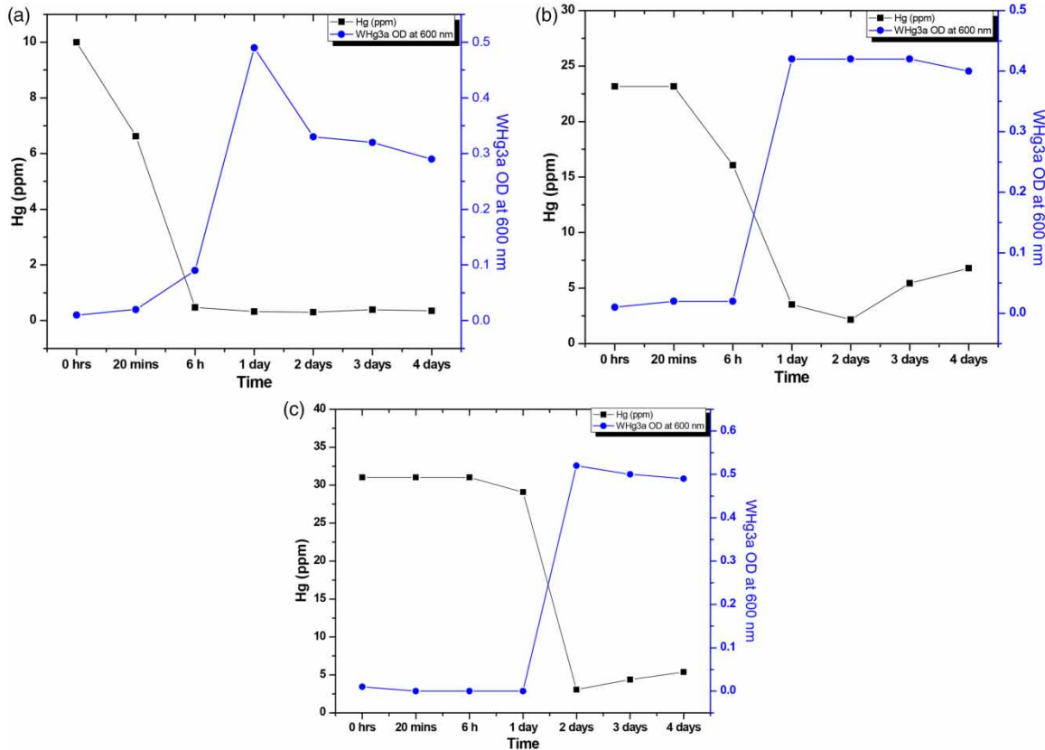
Figure 4 | The growth and mercury removed by bacteria at (a) 10 ppm of mercury, (b) 20 ppm of mercury and (c) 50 ppm of mercury.
