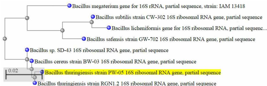
Figure 3 | Phylogenetic tree of the mercury resistant isolate prepared using the neighbour-joining method.
