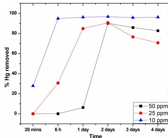
Figure 5 | Percentage removal of mercury by WHg3a isolate at varying concentrations of mercury.
