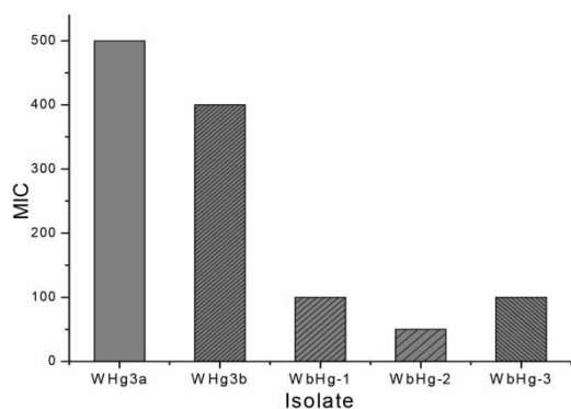
Figure 1 | MIC (ppm) of mercury for the isolated bacteria.
