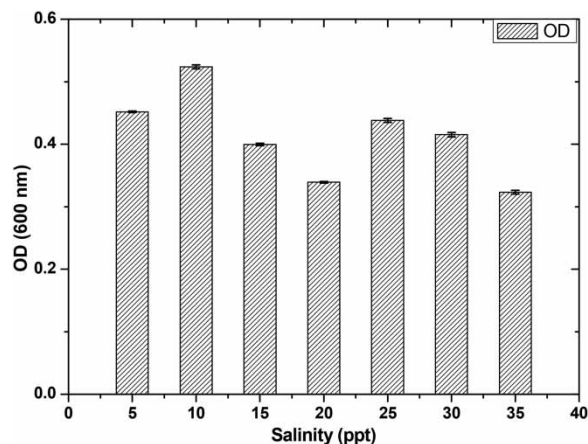
Figure 2 | Optical density of the WHg3a isolate at different salt concentrations at 600 nm.
